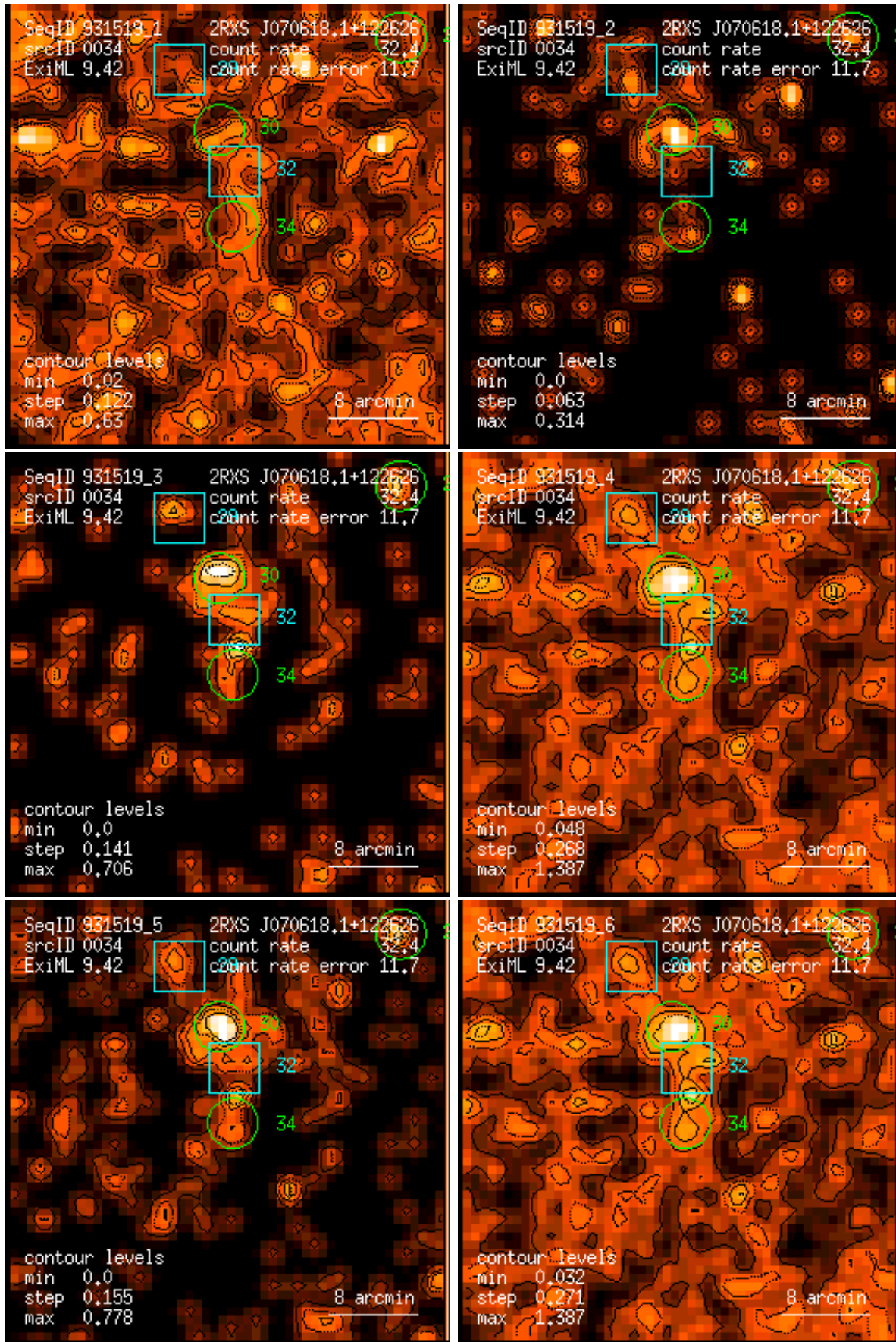
Figure 34: RASS 931519: detection 0034: band rate images, Gaussian filter: (1) PSPC channels 11 – 41, (2) 52 – 90, (3) 91 – 201, (4) 11 – 235, (5) 52 – 201, (6) 11 – 201. Broad band rates in counts/ks. Band rate contour levels in counts/ks/arcmin 2 .
