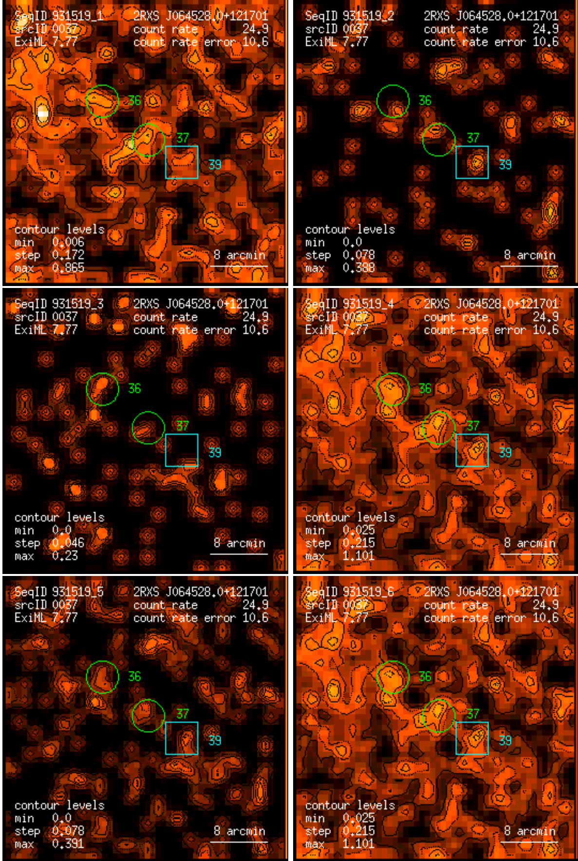
Figure 37: RASS 931519: detection 0037: band rate images, Gaussian filter: (1) PSPC channels 11 – 41, (2) 52 – 90, (3) 91 – 201, (4) 11 – 235, (5) 52 – 201, (6) 11 – 201. Broad band rates in counts/ks. Band rate contour levels in counts/ks/arcmin 2 .
