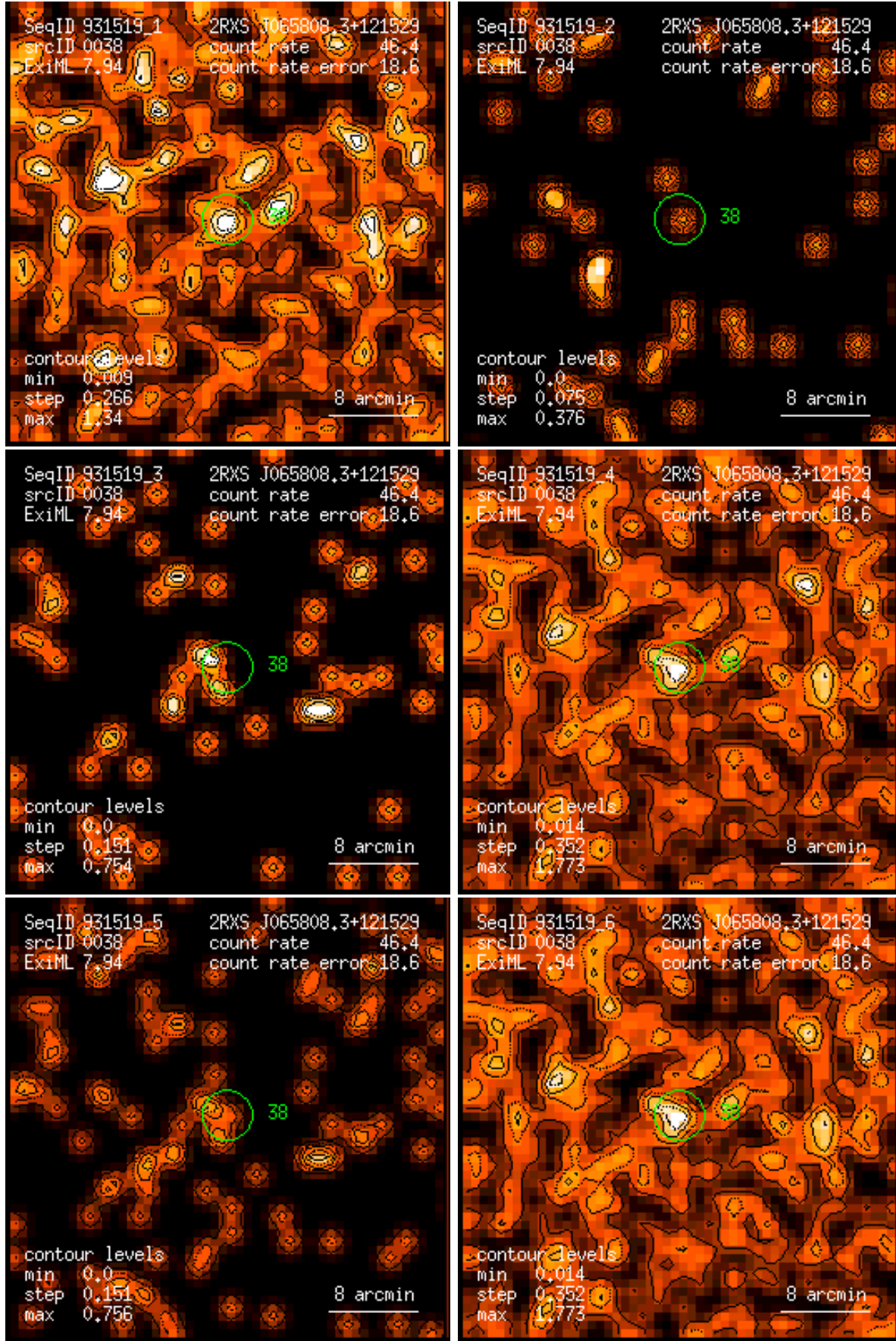
Figure 38: RASS 931519: detection 0038: band rate images, Gaussian filter: (1) PSPC channels 11 – 41, (2) 52 – 90, (3) 91 – 201, (4) 11 – 235, (5) 52 – 201, (6) 11 – 201. Broad band rates in counts/ks. Band rate contour levels in counts/ks/arcmin 2 .
