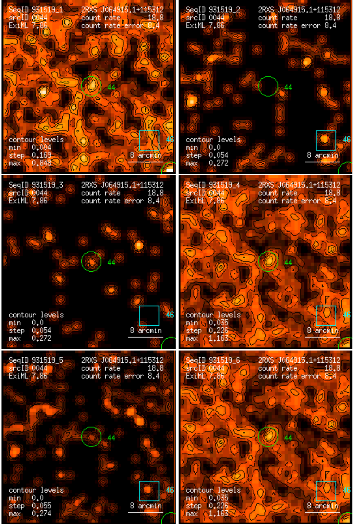
Figure 44: RASS 931519: detection 0044: band rate images, Gaussian filter: (1) PSPC channels 11 – 41, (2) 52 – 90, (3) 91 – 201, (4) 11 – 235, (5) 52 – 201, (6) 11 – 201. Broad band rates in counts/ks. Band rate contour levels in counts/ks/arcmin 2 .
