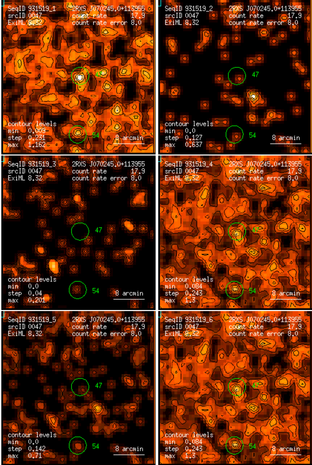
Figure 47: RASS 931519: detection 0047: band rate images, Gaussian filter: (1) PSPC channels 11 – 41, (2) 52 – 90, (3) 91 – 201, (4) 11 – 235, (5) 52 – 201, (6) 11 – 201. Broad band rates in counts/ks. Band rate contour levels in counts/ks/arcmin 2 .
