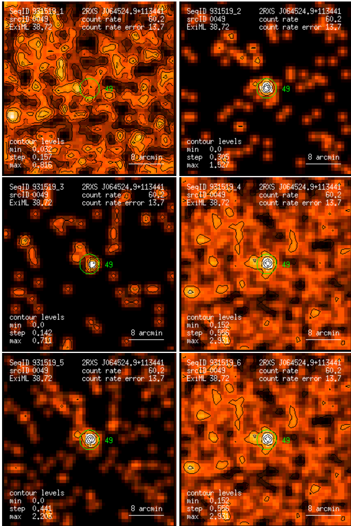
Figure 49: RASS 931519: detection 0049: band rate images, Gaussian filter: (1) PSPC channels 11 – 41, (2) 52 – 90, (3) 91 – 201, (4) 11 – 235, (5) 52 – 201, (6) 11 – 201. Broad band rates in counts/ks. Band rate contour levels in counts/ks/arcmin 2 .
