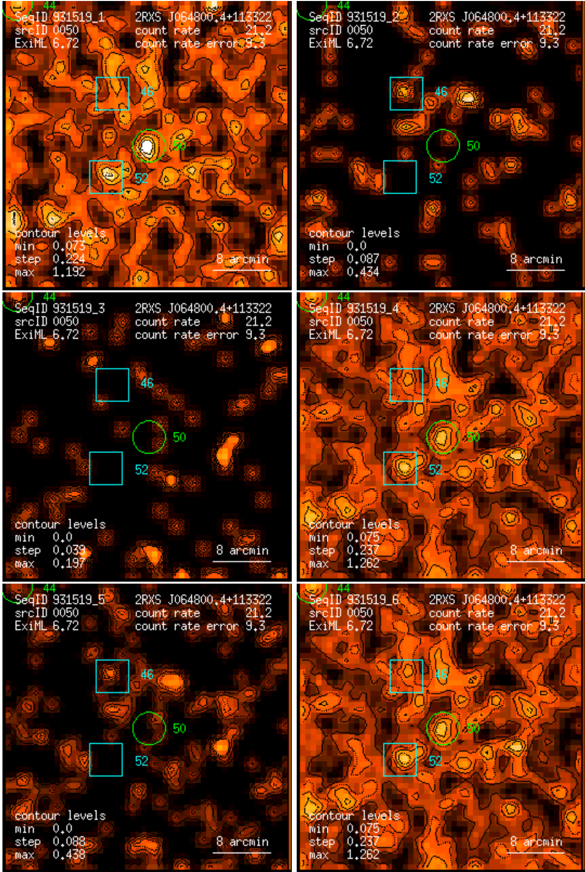
Figure 50: RASS 931519: detection 0050: band rate images, Gaussian filter: (1) PSPC channels 11 – 41, (2) 52 – 90, (3) 91 – 201, (4) 11 – 235, (5) 52 – 201, (6) 11 – 201. Broad band rates in counts/ks. Band rate contour levels in counts/ks/arcmin 2 .
