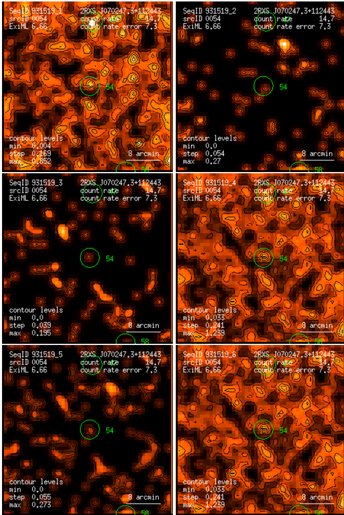
Figure 54: RASS 931519: detection 0054: band rate images, Gaussian filter: (1) PSPC channels 11 – 41, (2) 52 – 90, (3) 91 – 201, (4) 11 – 235, (5) 52 – 201, (6) 11 – 201. Broad band rates in counts/ks. Band rate contour levels in counts/ks/arcmin 2 .
