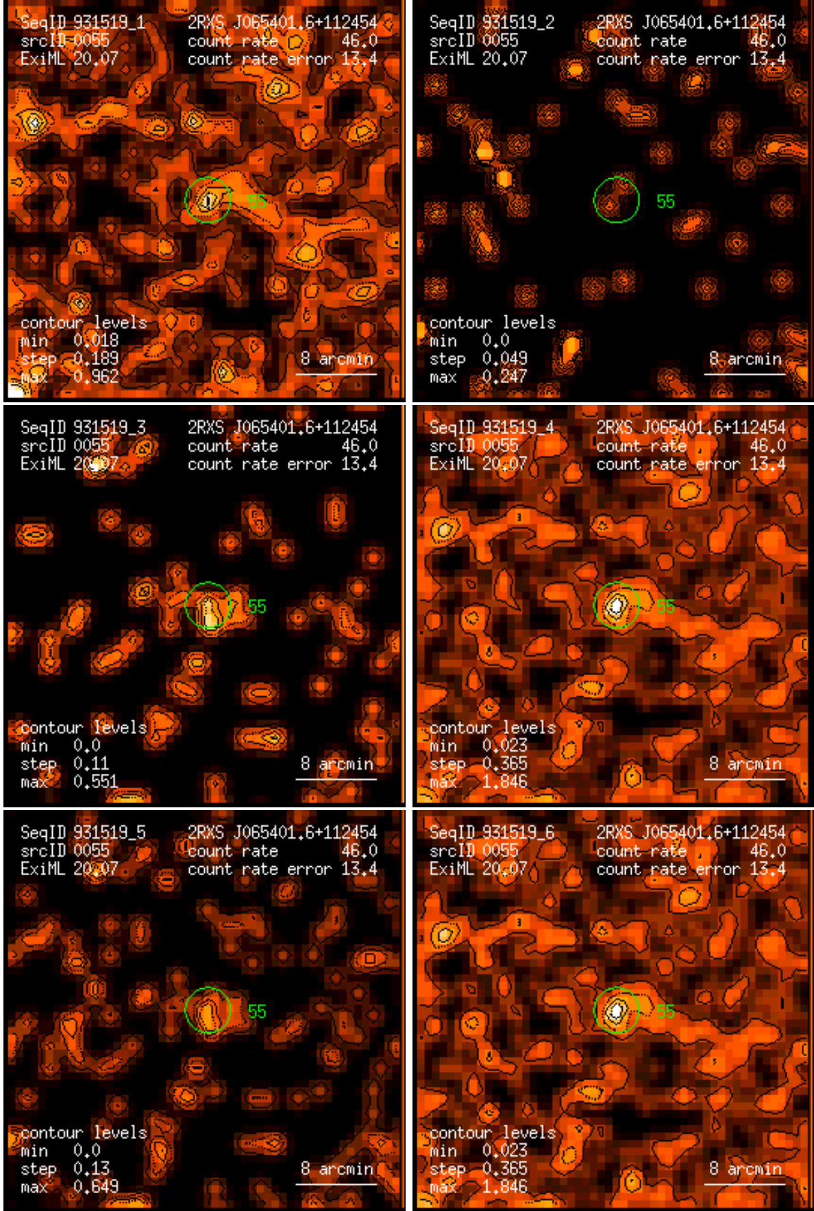
Figure 55: RASS 931519: detection 0055: band rate images, Gaussian filter: (1) PSPC channels 11 – 41, (2) 52 – 90, (3) 91 – 201, (4) 11 – 235, (5) 52 – 201, (6) 11 – 201. Broad band rates in counts/ks. Band rate contour levels in counts/ks/arcmin 2 .
