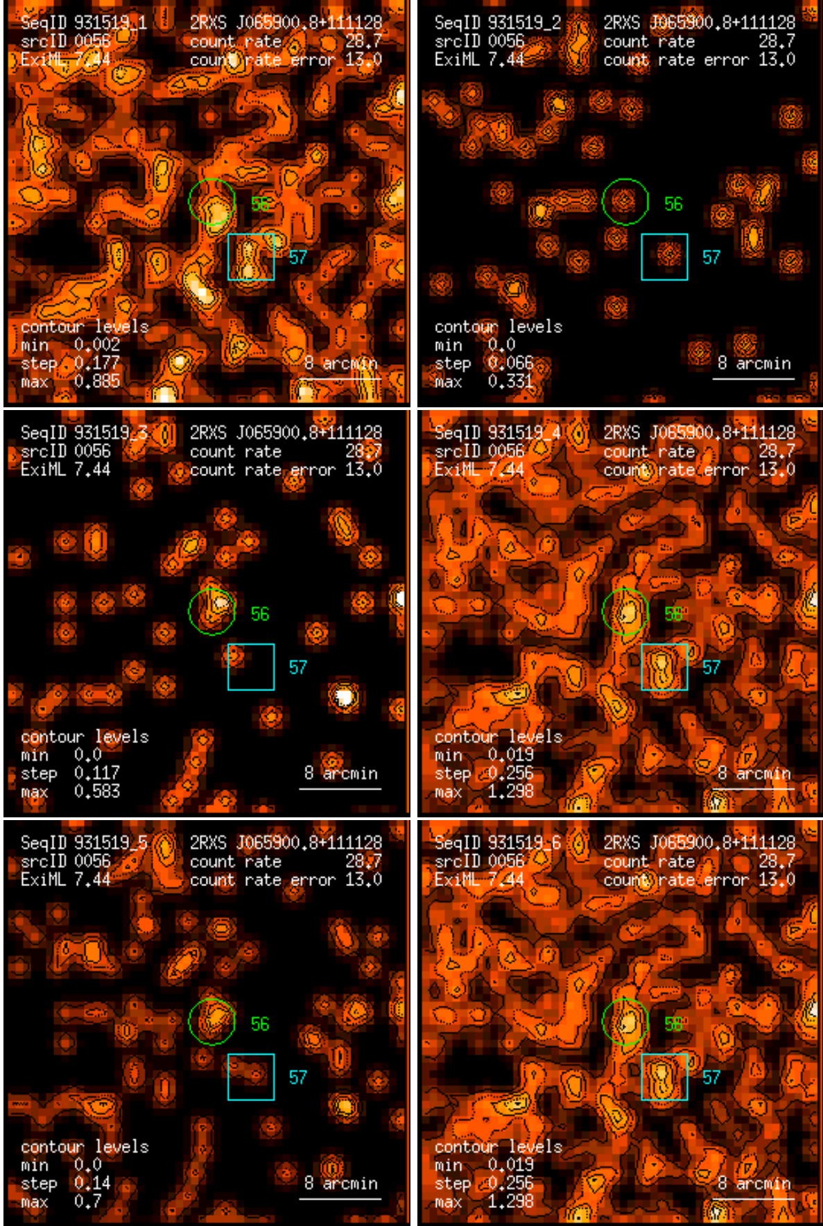
Figure 56: RASS 931519: detection 0056: band rate images, Gaussian filter: (1) PSPC channels 11 – 41, (2) 52 – 90, (3) 91 – 201, (4) 11 – 235, (5) 52 – 201, (6) 11 – 201. Broad band rates in counts/ks. Band rate contour levels in counts/ks/arcmin 2 .
