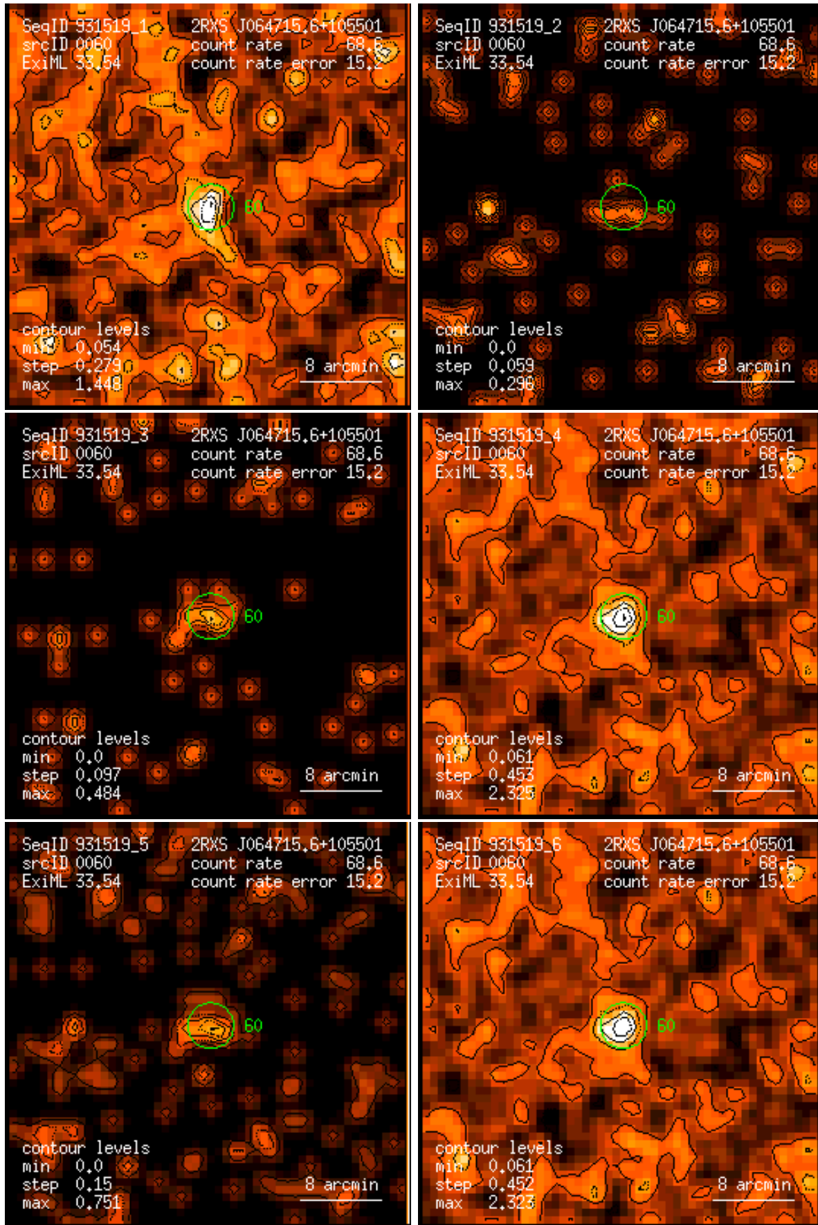
Figure 60: RASS 931519: detection 0060: band rate images, Gaussian filter: (1) PSPC channels 11 – 41, (2) 52 – 90, (3) 91 – 201, (4) 11 – 235, (5) 52 – 201, (6) 11 – 201. Broad band rates in counts/ks. Band rate contour levels in counts/ks/arcmin 2 .
