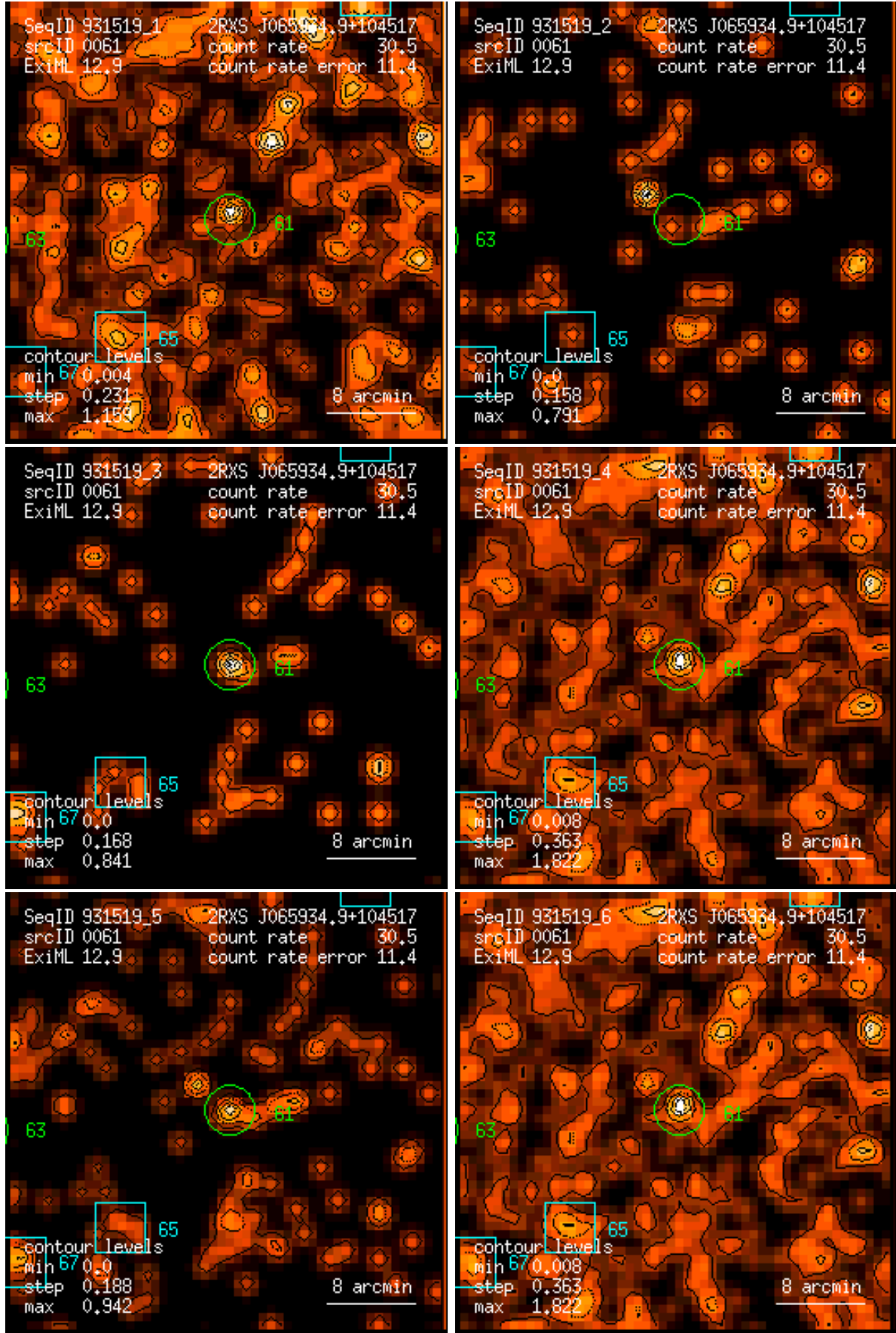
Figure 61: RASS 931519: detection 0061: band rate images, Gaussian filter: (1) PSPC channels 11 – 41, (2) 52 – 90, (3) 91 – 201, (4) 11 – 235, (5) 52 – 201, (6) 11 – 201. Broad band rates in counts/ks. Band rate contour levels in counts/ks/arcmin 2 .
