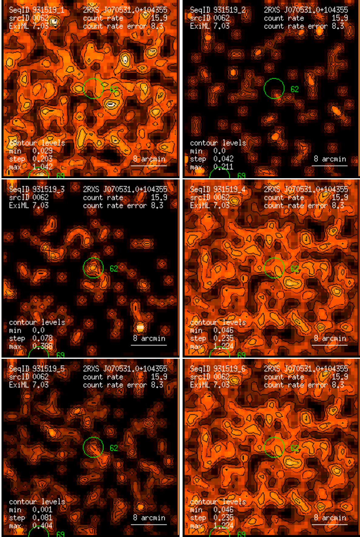
Figure 62: RASS 931519: detection 0062: band rate images, Gaussian filter: (1) PSPC channels 11 – 41, (2) 52 – 90, (3) 91 – 201, (4) 11 – 235, (5) 52 – 201, (6) 11 – 201. Broad band rates in counts/ks. Band rate contour levels in counts/ks/arcmin 2 .
