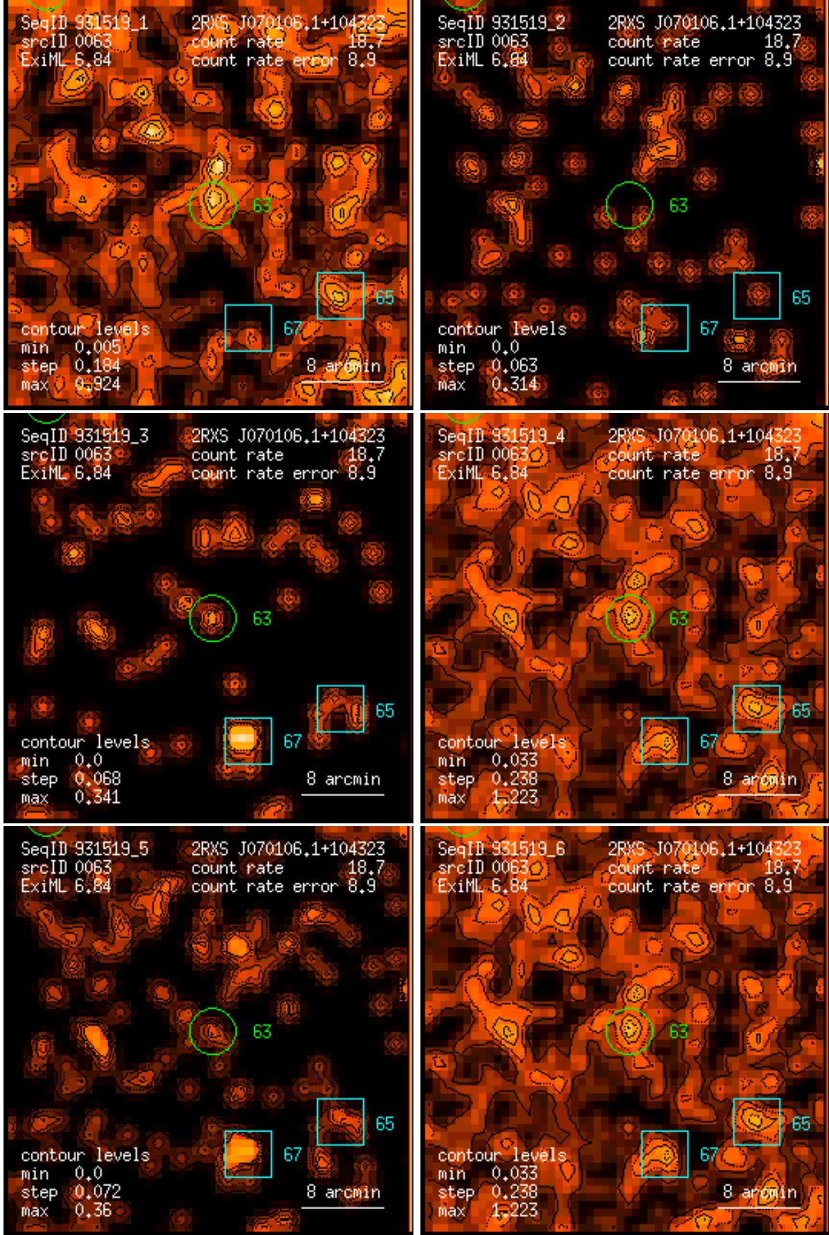
Figure 63: RASS 931519: detection 0063: band rate images, Gaussian filter: (1) PSPC channels 11 – 41, (2) 52 – 90, (3) 91 – 201, (4) 11 – 235, (5) 52 – 201, (6) 11 – 201. Broad band rates in counts/ks. Band rate contour levels in counts/ks/arcmin 2 .
