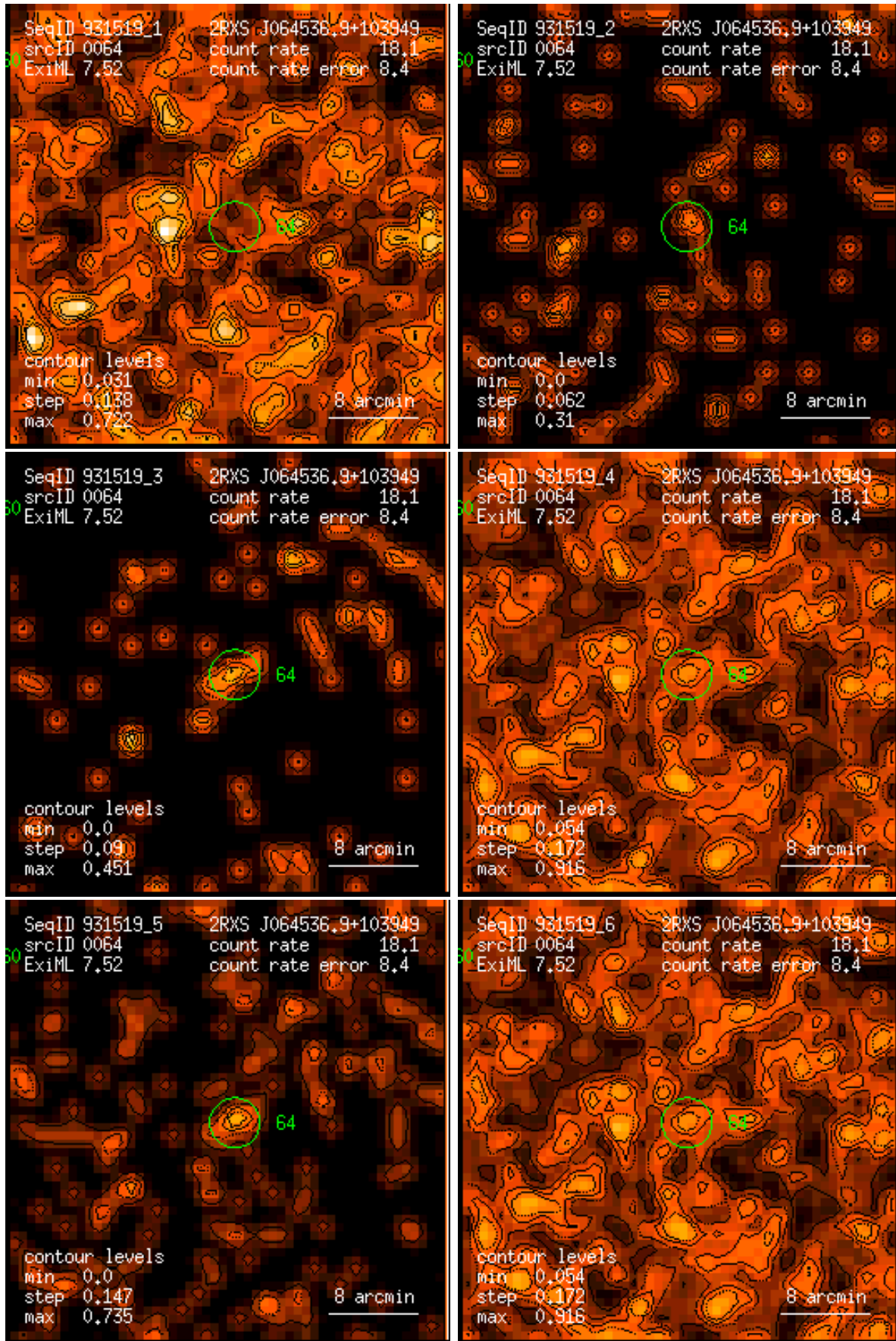
Figure 64: RASS 931519: detection 0064: band rate images, Gaussian filter: (1) PSPC channels 11 – 41, (2) 52 – 90, (3) 91 – 201, (4) 11 – 235, (5) 52 – 201, (6) 11 – 201. Broad band rates in counts/ks. Band rate contour levels in counts/ks/arcmin 2 .
