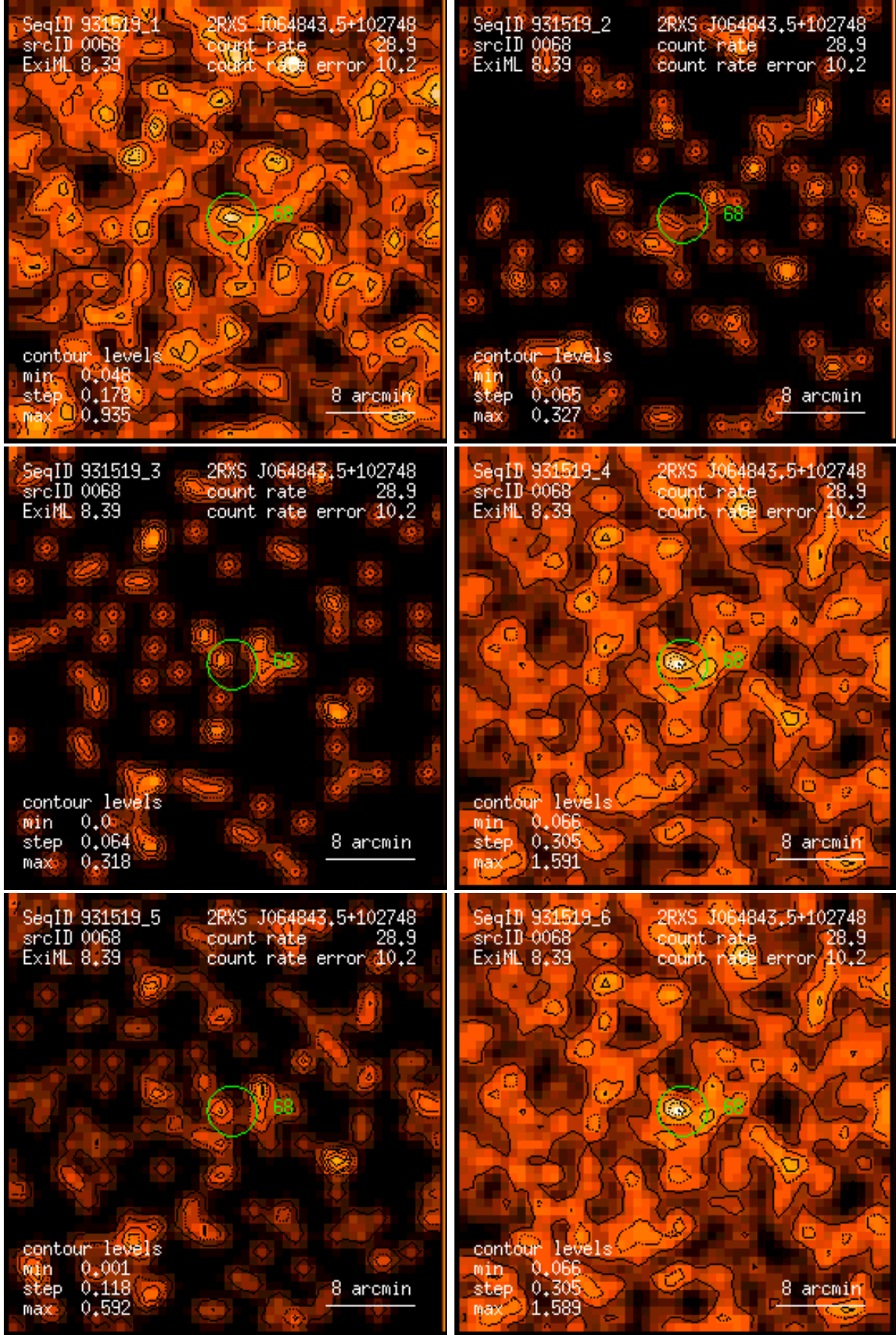
Figure 68: RASS 931519: detection 0068: band rate images, Gaussian filter: (1) PSPC channels 11 – 41, (2) 52 – 90, (3) 91 – 201, (4) 11 – 235, (5) 52 – 201, (6) 11 – 201. Broad band rates in counts/ks. Band rate contour levels in counts/ks/arcmin 2 .
