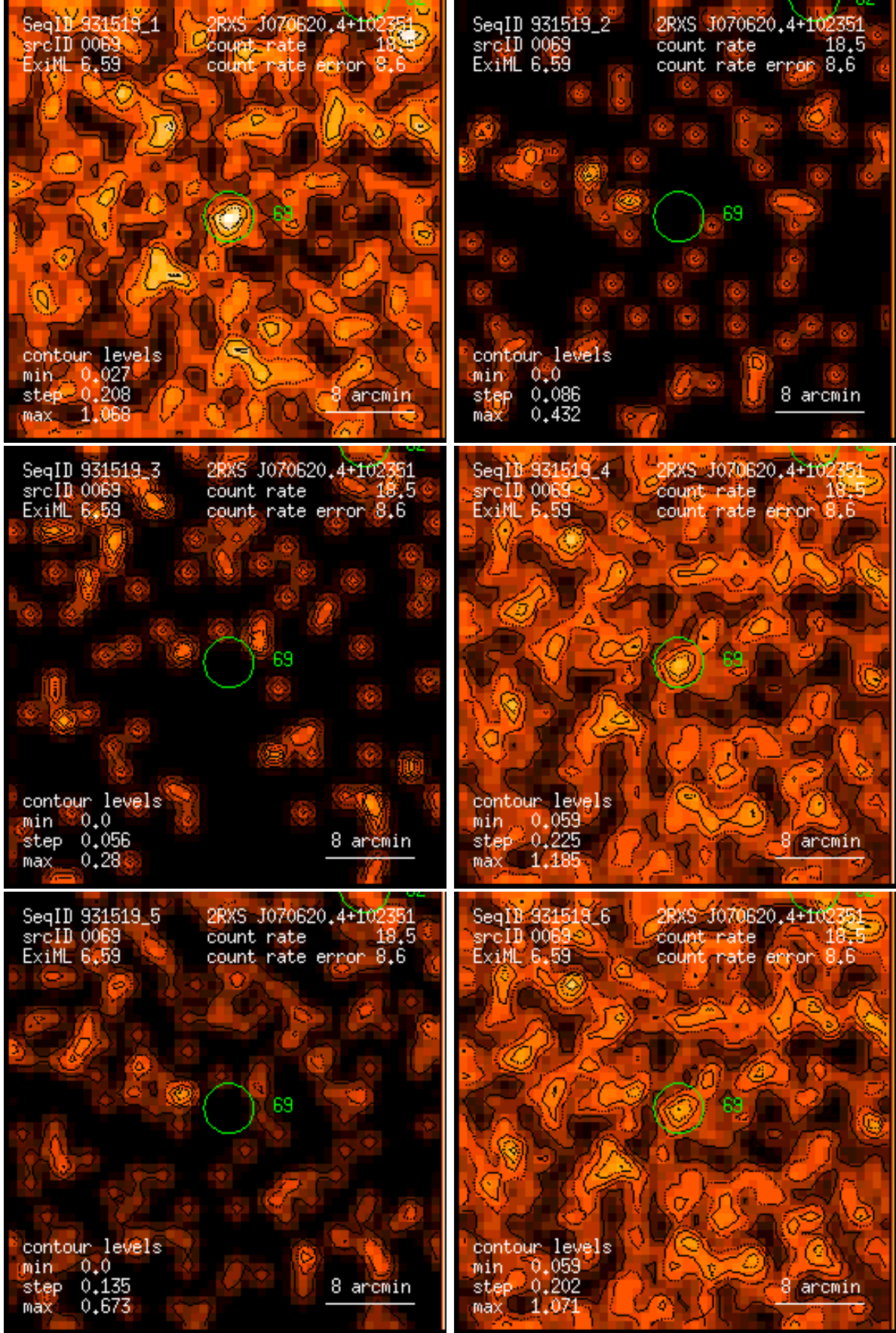
Figure 69: RASS 931519: detection 0069: band rate images, Gaussian filter: (1) PSPC channels 11 – 41, (2) 52 – 90, (3) 91 – 201, (4) 11 – 235, (5) 52 – 201, (6) 11 – 201. Broad band rates in counts/ks. Band rate contour levels in counts/ks/arcmin 2 .
