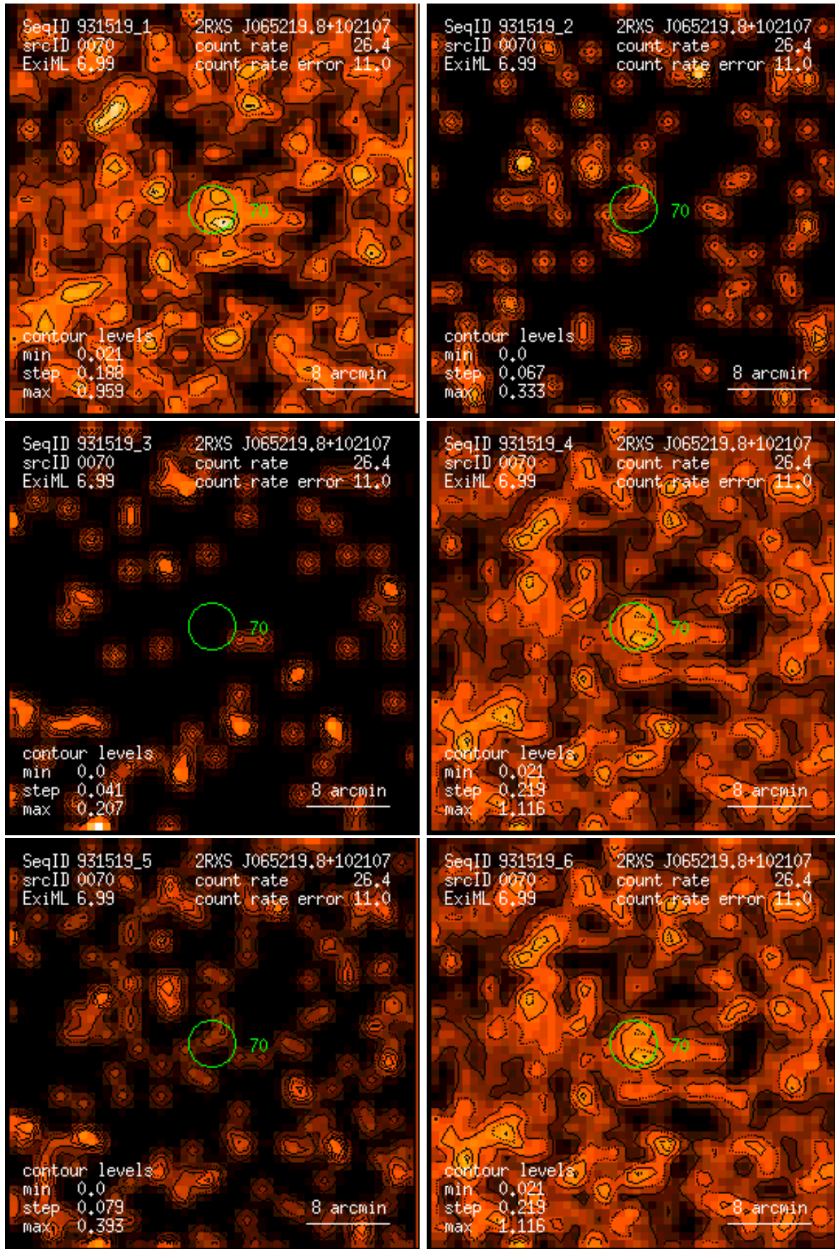
Figure 70: RASS 931519: detection 0070: band rate images, Gaussian filter: (1) PSPC channels 11 – 41, (2) 52 – 90, (3) 91 – 201, (4) 11 – 235, (5) 52 – 201, (6) 11 – 201. Broad band rates in counts/ks. Band rate contour levels in counts/ks/arcmin 2 .
