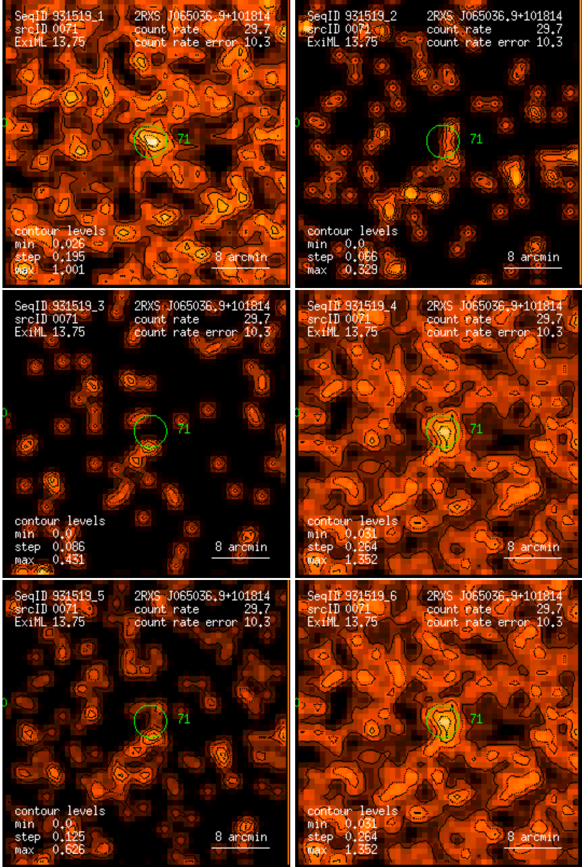
Figure 71: RASS 931519: detection 0071: band rate images, Gaussian filter: (1) PSPC channels 11 – 41, (2) 52 – 90, (3) 91 – 201, (4) 11 – 235, (5) 52 – 201, (6) 11 – 201. Broad band rates in counts/ks. Band rate contour levels in counts/ks/arcmin 2 .
