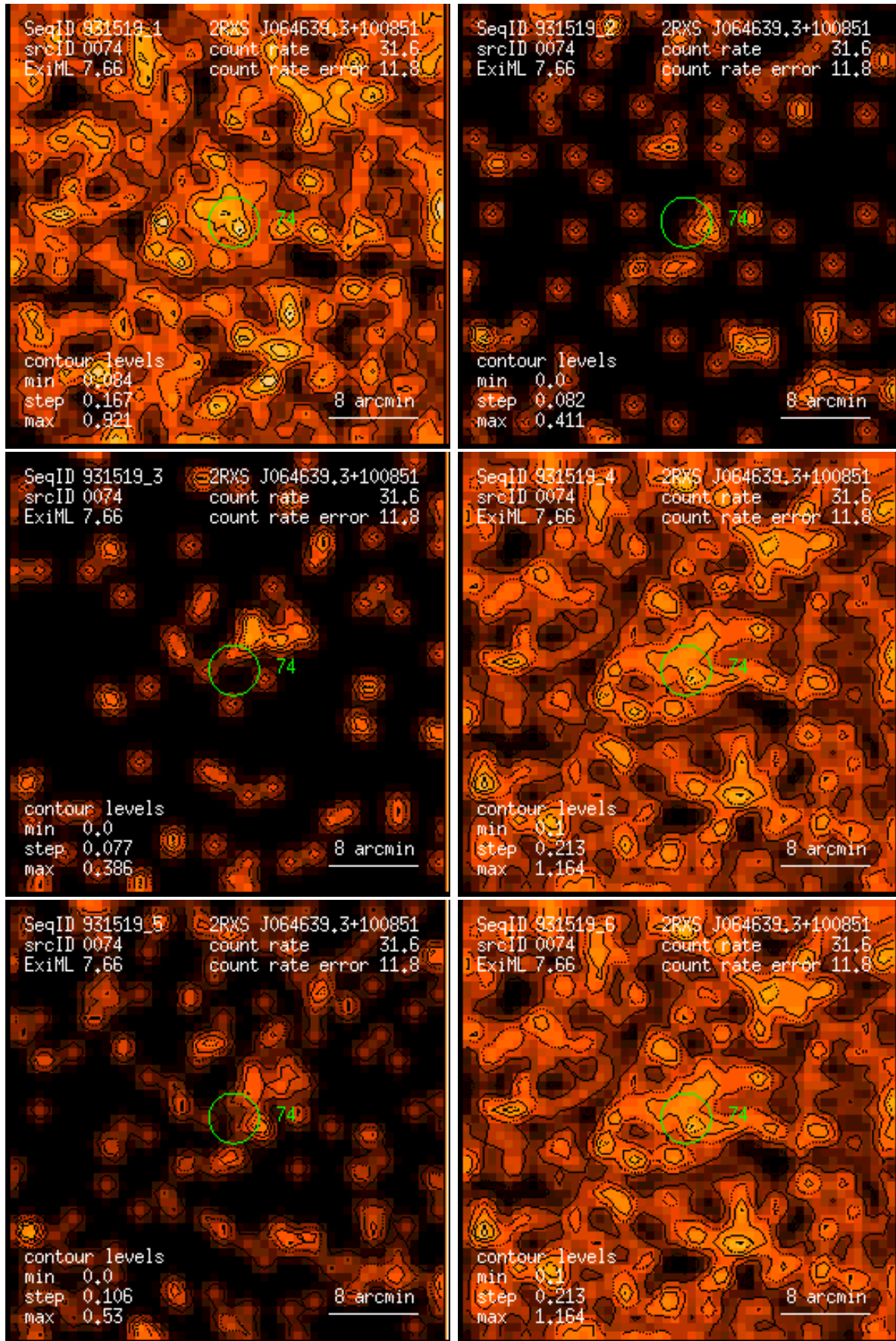
Figure 74: RASS 931519: detection 0074: band rate images, Gaussian filter: (1) PSPC channels 11 – 41, (2) 52 – 90, (3) 91 – 201, (4) 11 – 235, (5) 52 – 201, (6) 11 – 201. Broad band rates in counts/ks. Band rate contour levels in counts/ks/arcmin 2 .
