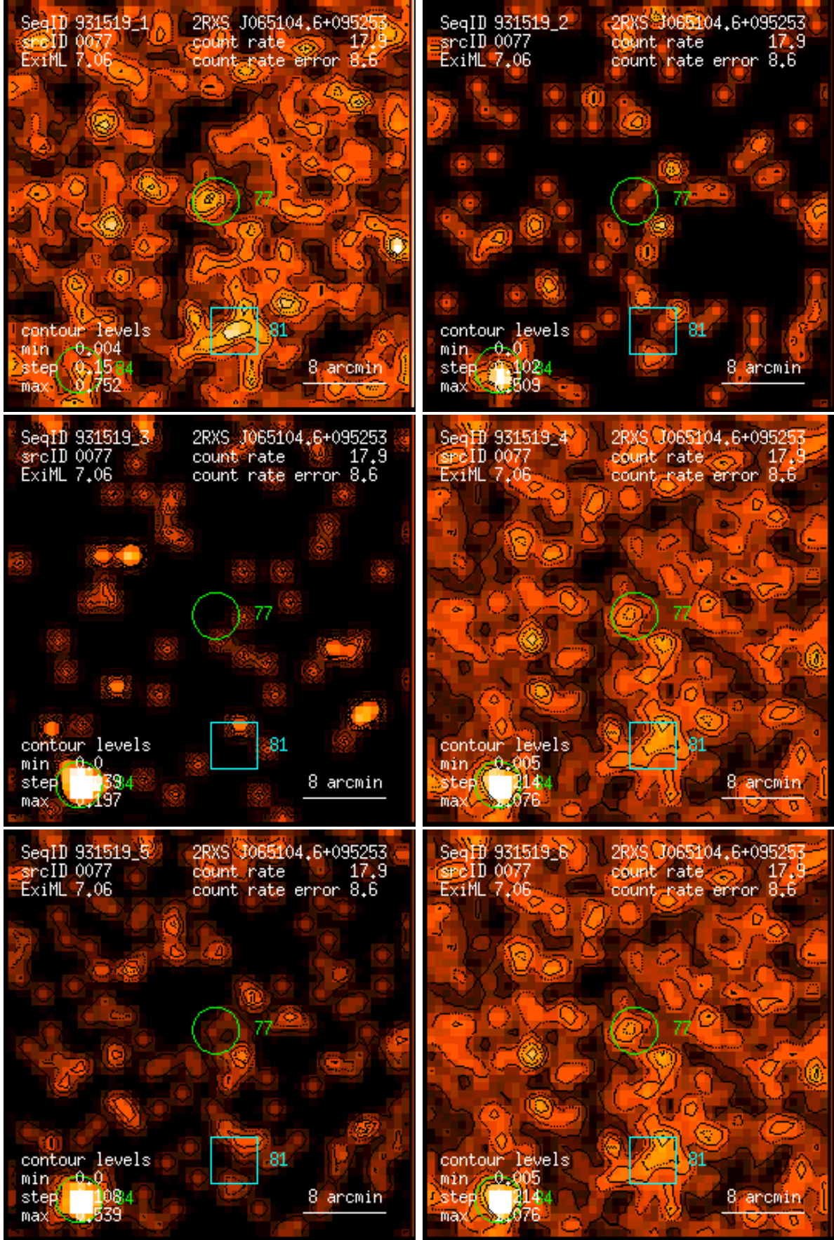
Figure 77: RASS 931519: detection 0077: band rate images, Gaussian filter: (1) PSPC channels 11 – 41, (2) 52 – 90, (3) 91 – 201, (4) 11 – 235, (5) 52 – 201, (6) 11 – 201. Broad band rates in counts/ks. Band rate contour levels in counts/ks/arcmin 2 .
