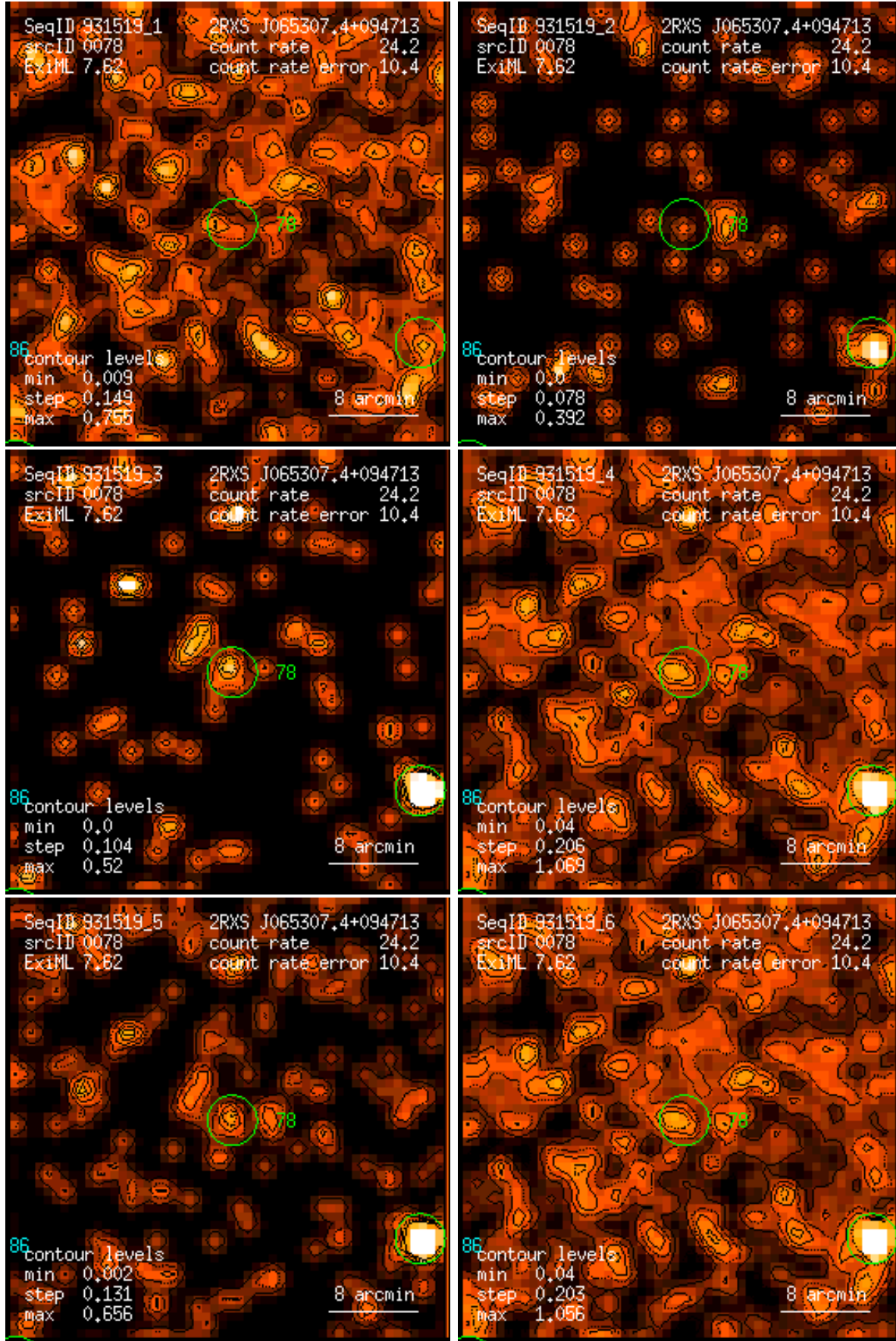
Figure 78: RASS 931519: detection 0078: band rate images, Gaussian filter: (1) PSPC channels 11 – 41, (2) 52 – 90, (3) 91 – 201, (4) 11 – 235, (5) 52 – 201, (6) 11 – 201. Broad band rates in counts/ks. Band rate contour levels in counts/ks/arcmin 2 .
