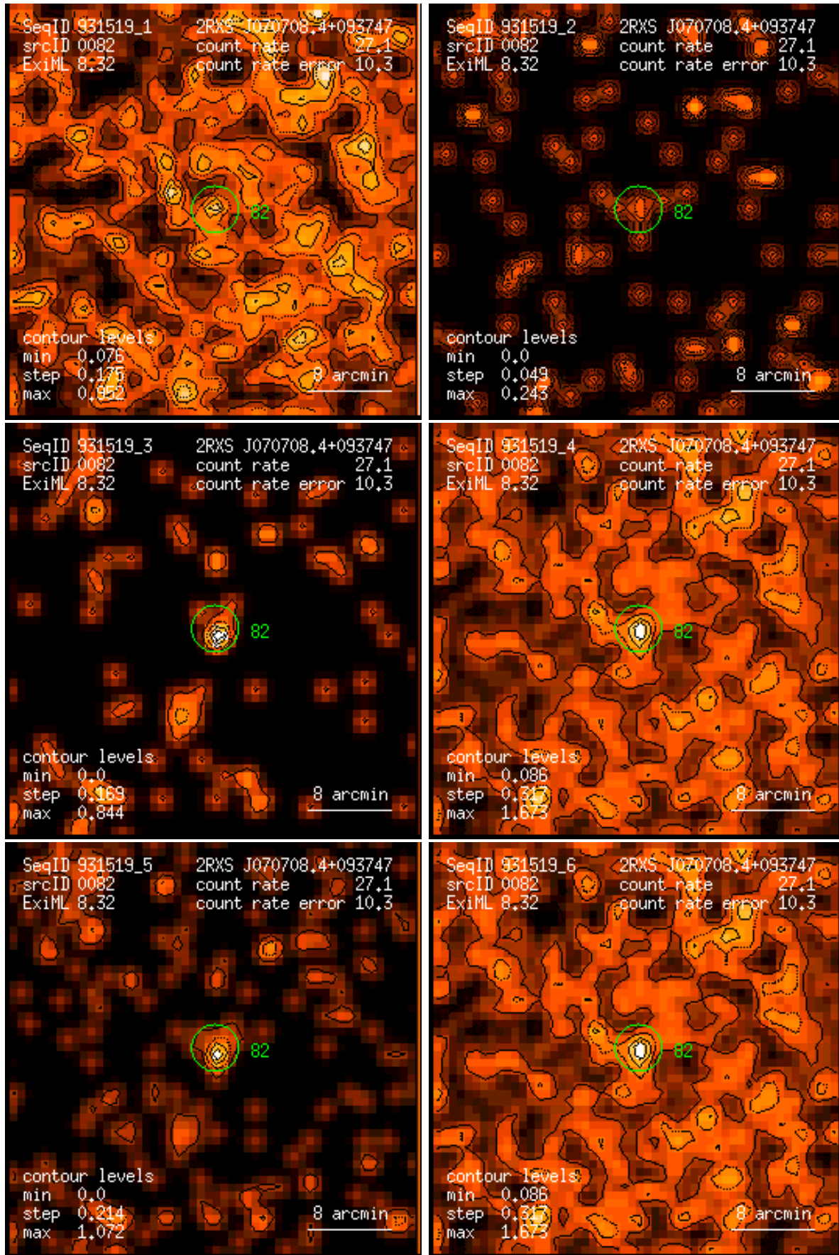
Figure 82: RASS 931519: detection 0082: band rate images, Gaussian filter: (1) PSPC channels 11 – 41, (2) 52 – 90, (3) 91 – 201, (4) 11 – 235, (5) 52 – 201, (6) 11 – 201. Broad band rates in counts/ks. Band rate contour levels in counts/ks/arcmin 2 .
