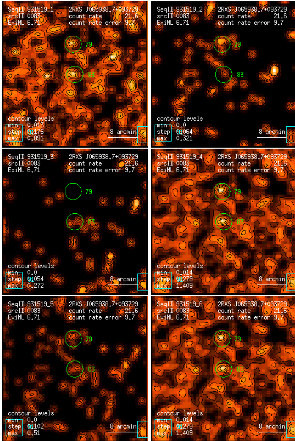
Figure 83: RASS 931519: detection 0083: band rate images, Gaussian filter: (1) PSPC channels 11 – 41, (2) 52 – 90, (3) 91 – 201, (4) 11 – 235, (5) 52 – 201, (6) 11 – 201. Broad band rates in counts/ks. Band rate contour levels in counts/ks/arcmin 2 .
