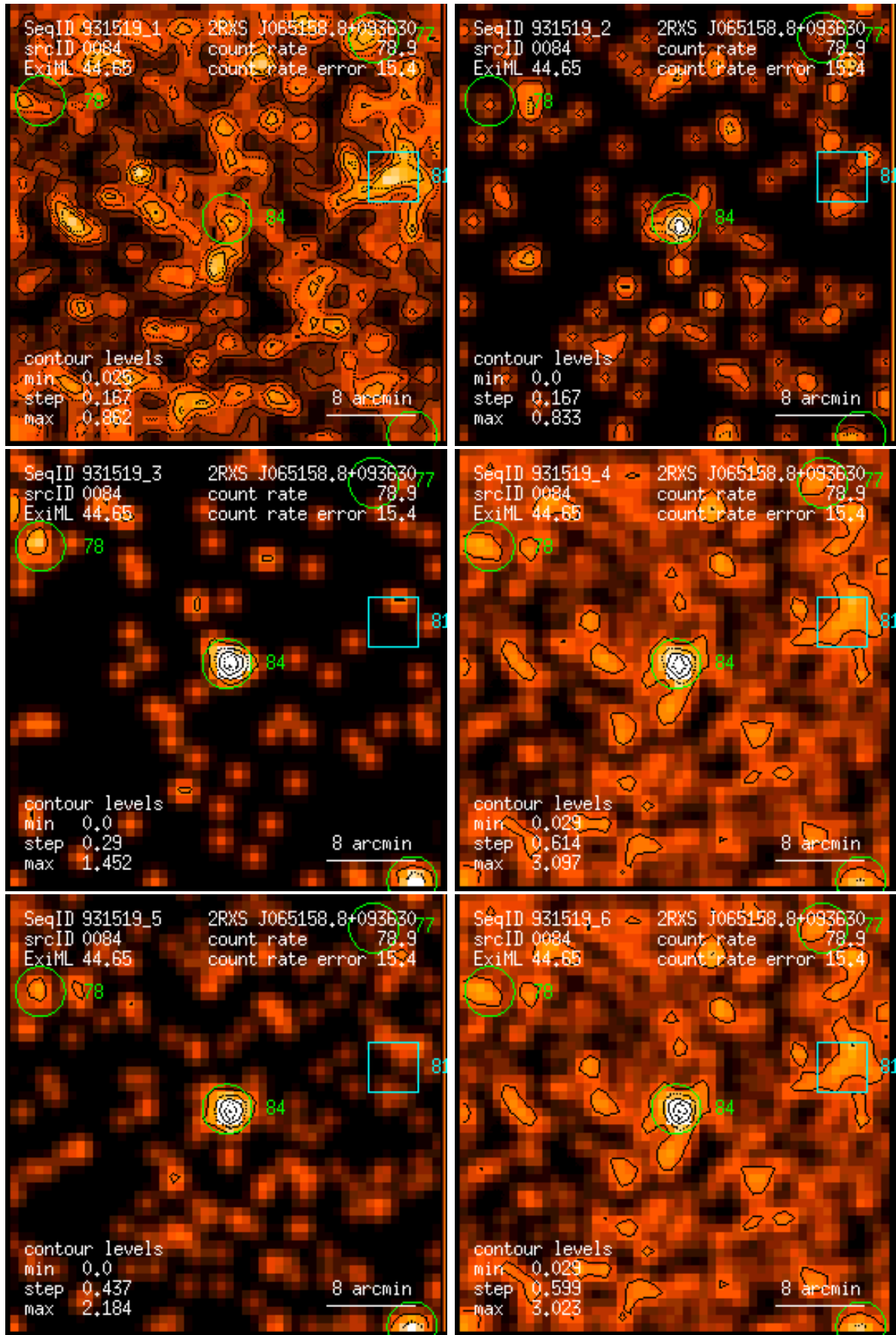
Figure 84: RASS 931519: detection 0084: band rate images, Gaussian filter: (1) PSPC channels 11 – 41, (2) 52 – 90, (3) 91 – 201, (4) 11 – 235, (5) 52 – 201, (6) 11 – 201. Broad band rates in counts/ks. Band rate contour levels in counts/ks/arcmin 2 .
