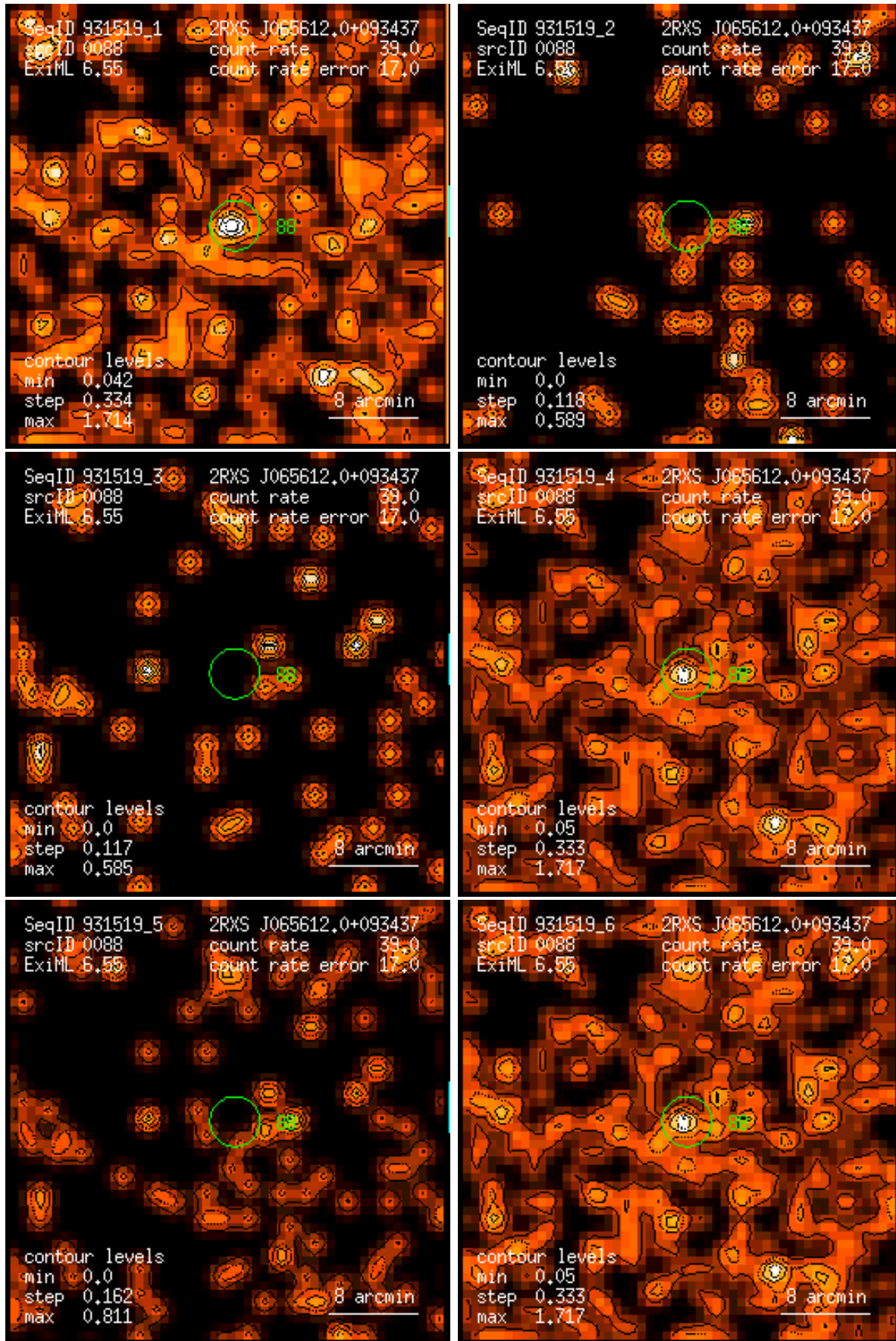
Figure 88: RASS 931519: detection 0088: band rate images, Gaussian filter: (1) PSPC channels 11 – 41, (2) 52 – 90, (3) 91 – 201, (4) 11 – 235, (5) 52 – 201, (6) 11 – 201. Broad band rates in counts/ks. Band rate contour levels in counts/ks/arcmin 2 .
