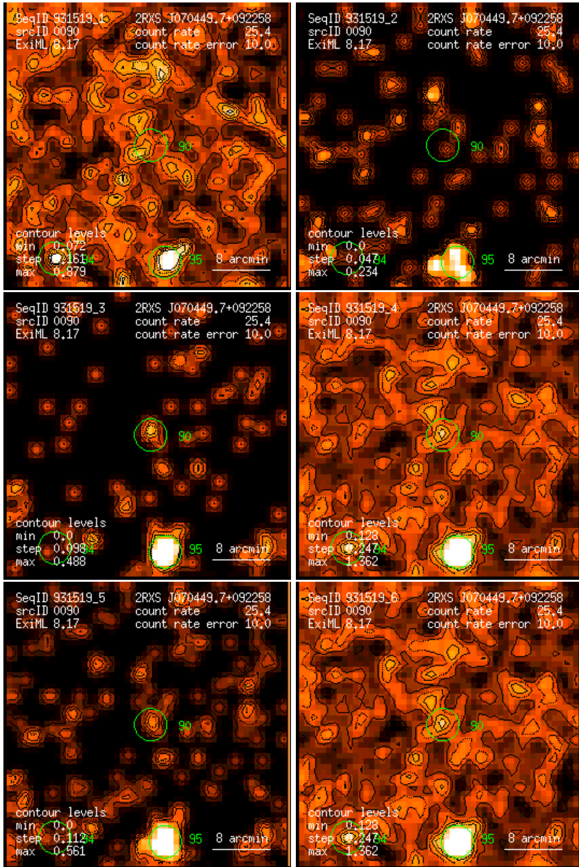
Figure 90: RASS 931519: detection 0090: band rate images, Gaussian filter: (1) PSPC channels 11 – 41, (2) 52 – 90, (3) 91 – 201, (4) 11 – 235, (5) 52 – 201, (6) 11 – 201. Broad band rates in counts/ks. Band rate contour levels in counts/ks/arcmin 2 .
