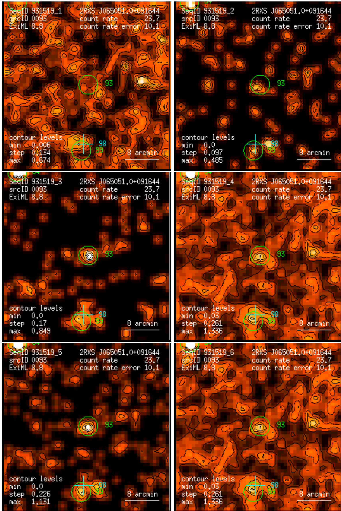
Figure 93: RASS 931519: detection 0093: band rate images, Gaussian filter: (1) PSPC channels 11 – 41, (2) 52 – 90, (3) 91 – 201, (4) 11 – 235, (5) 52 – 201, (6) 11 – 201. Broad band rates in counts/ks. Band rate contour levels in counts/ks/arcmin 2 .
