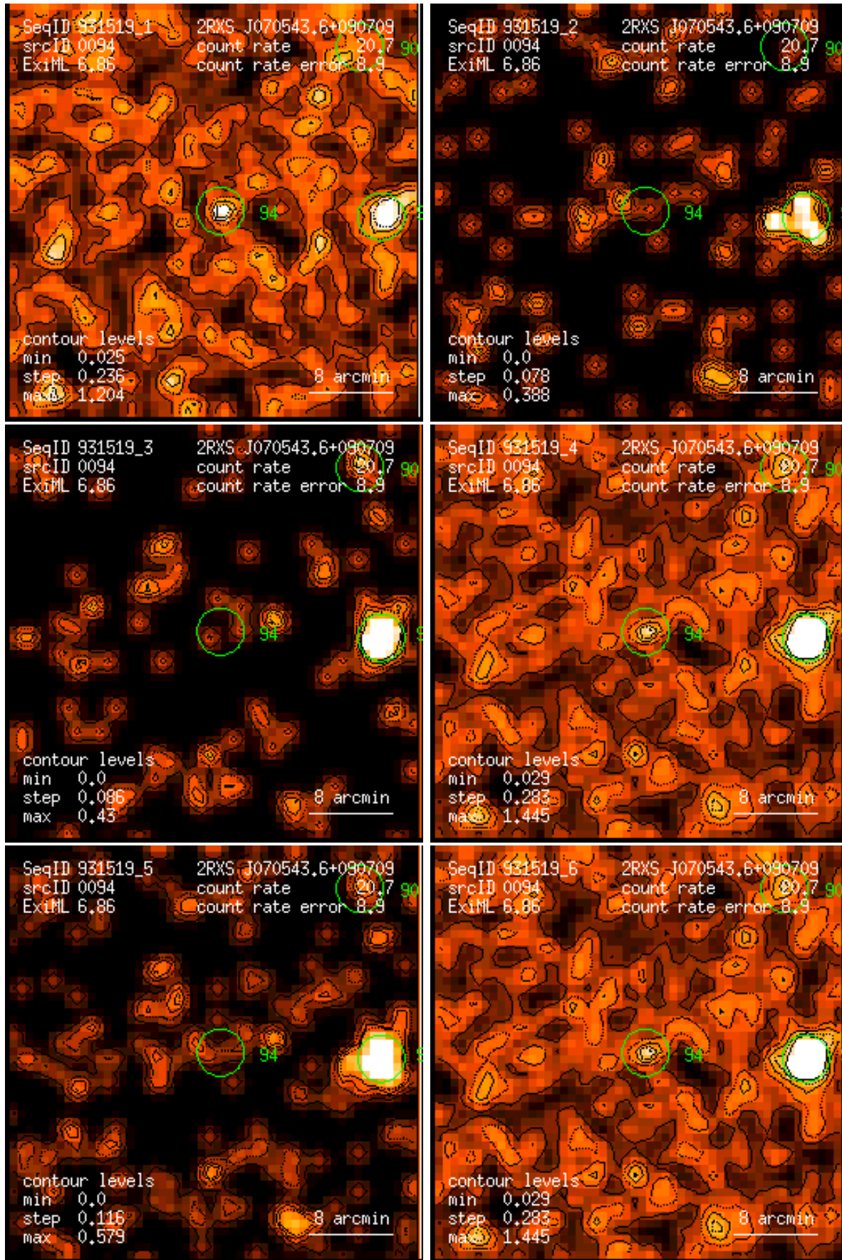
Figure 94: RASS 931519: detection 0094: band rate images, Gaussian filter: (1) PSPC channels 11 – 41, (2) 52 – 90, (3) 91 – 201, (4) 11 – 235, (5) 52 – 201, (6) 11 – 201. Broad band rates in counts/ks. Band rate contour levels in counts/ks/arcmin 2 .
