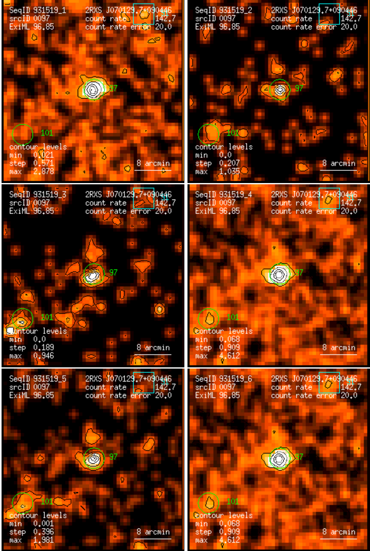
Figure 97: RASS 931519: detection 0097: band rate images, Gaussian filter: (1) PSPC channels 11 – 41, (2) 52 – 90, (3) 91 – 201, (4) 11 – 235, (5) 52 – 201, (6) 11 – 201. Broad band rates in counts/ks. Band rate contour levels in counts/ks/arcmin 2 .
