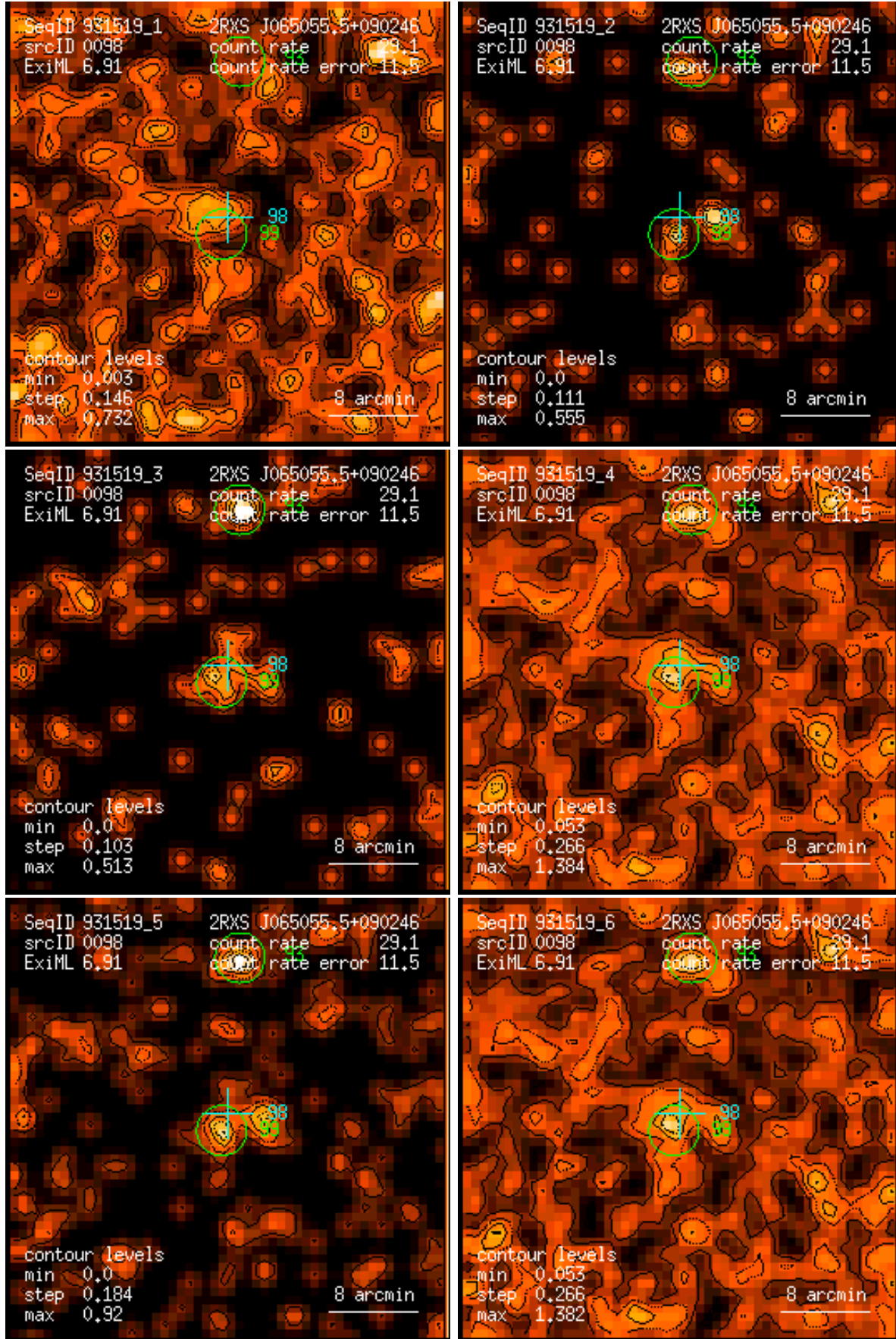
Figure 98: RASS 931519: detection 0098: band rate images, Gaussian filter: (1) PSPC channels 11 – 41, (2) 52 – 90, (3) 91 – 201, (4) 11 – 235, (5) 52 – 201, (6) 11 – 201. Broad band rates in counts/ks. Band rate contour levels in counts/ks/arcmin 2 .
