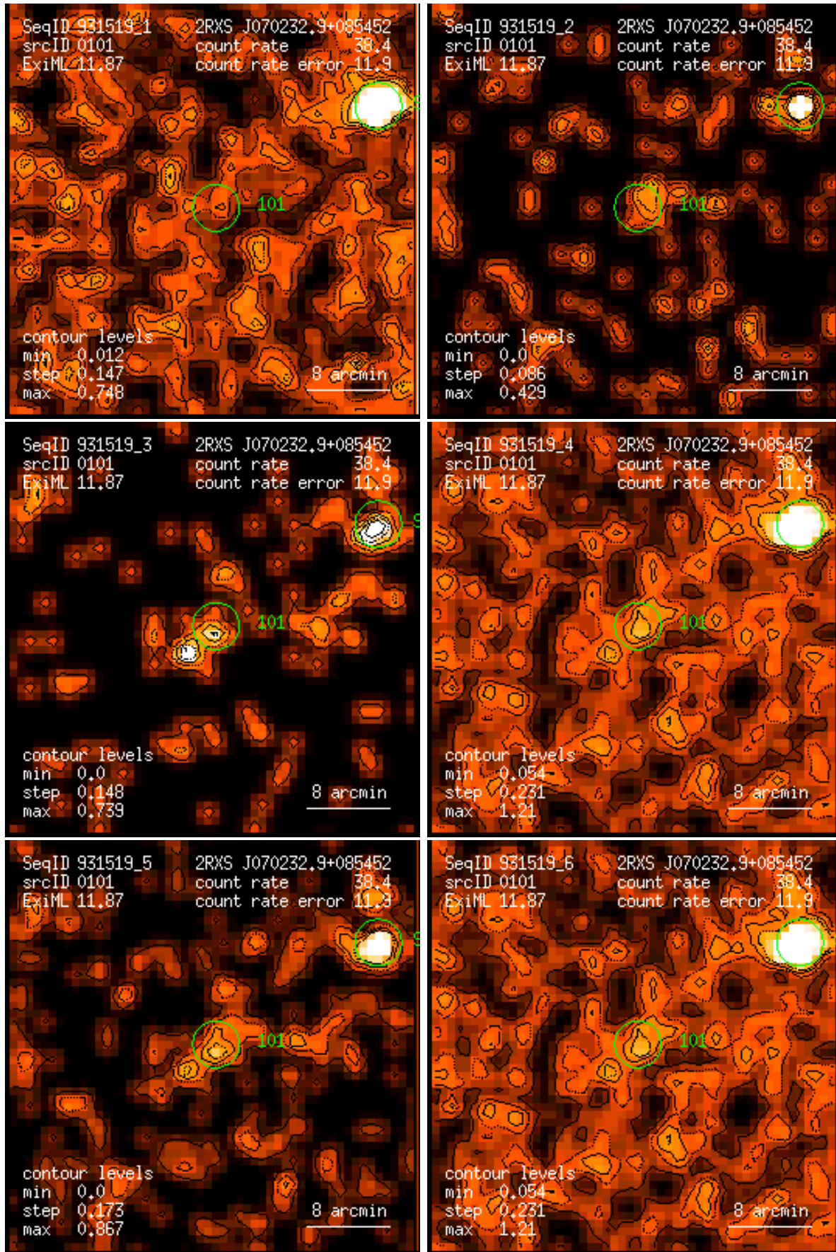
Figure 101: RASS 931519: detection 0101: band rate images, Gaussian filter: (1) PSPC channels 11 – 41, (2) 52 – 90, (3) 91 – 201, (4) 11 – 235, (5) 52 – 201, (6) 11 – 201. Broad band rates in counts/ks. Band rate contour levels in counts/ks/arcmin 2 .
