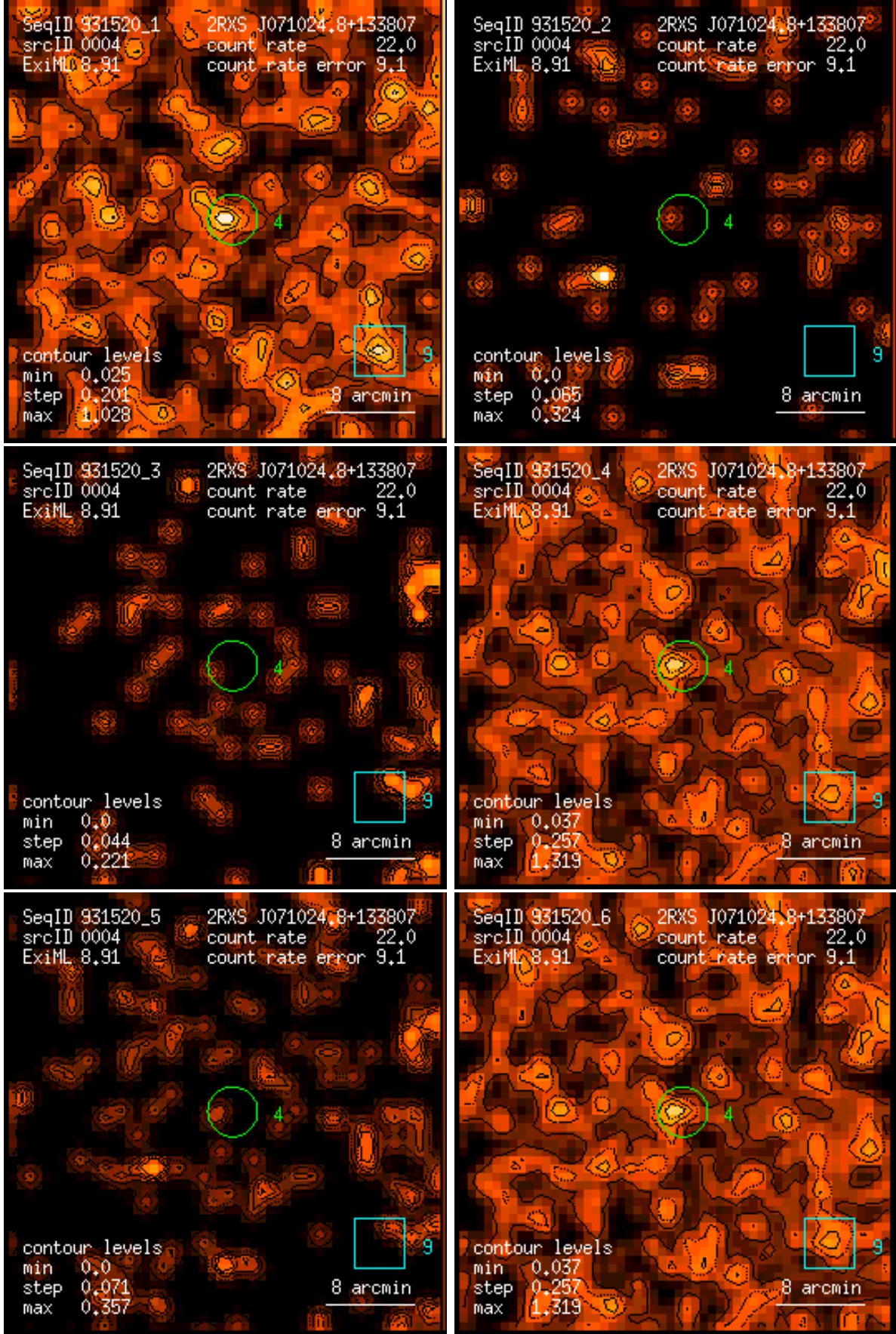
Figure 4: RASS 931520: detection 0004: band rate images, Gaussian filter: (1) PSPC channels 11 – 41, (2) 52 – 90, (3) 91 – 201, (4) 11 – 235, (5) 52 – 201, (6) 11 – 201. Broad band rates in counts/ks. Band rate contour levels in counts/ks/arcmin 2 .
