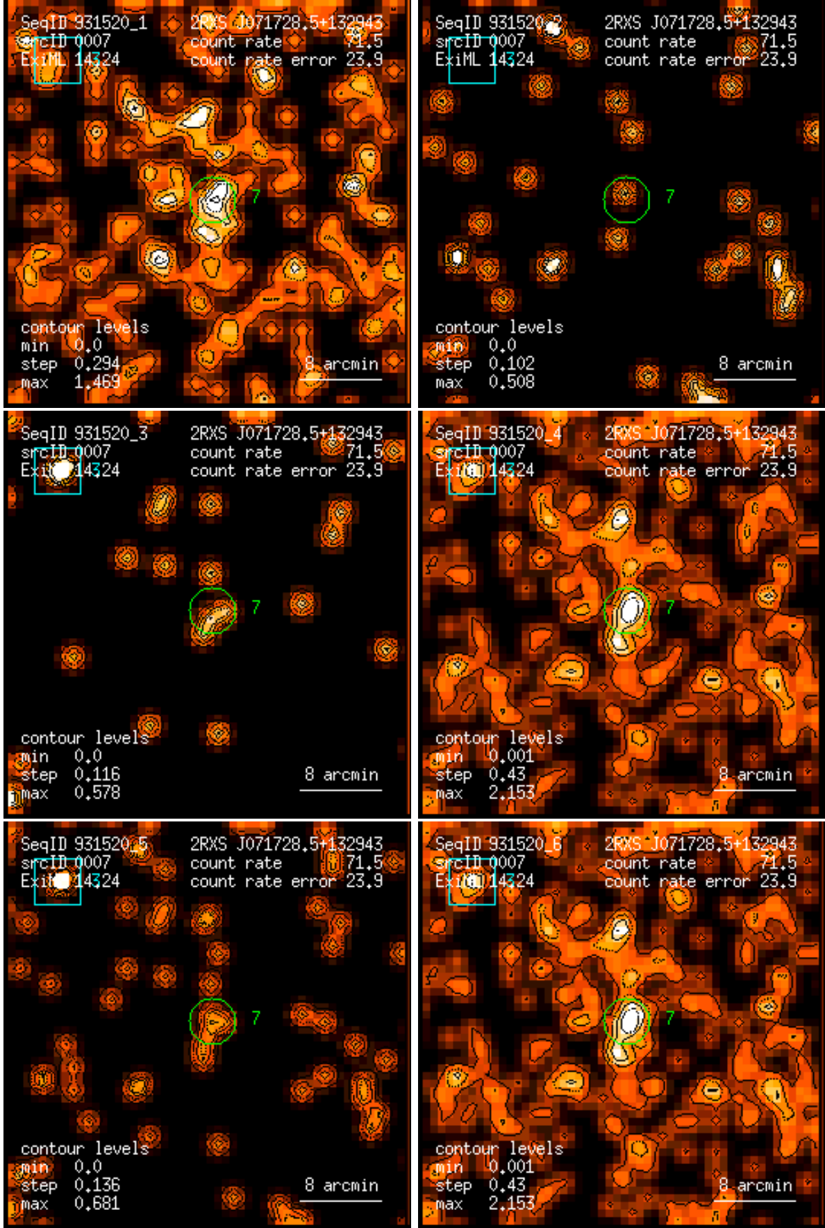
Figure 7: RASS 931520: detection 0007: band rate images, Gaussian filter: (1) PSPC channels 11 – 41, (2) 52 – 90, (3) 91 – 201, (4) 11 – 235, (5) 52 – 201, (6) 11 – 201. Broad band rates in counts/ks. Band rate contour levels in counts/ks/arcmin 2 .
