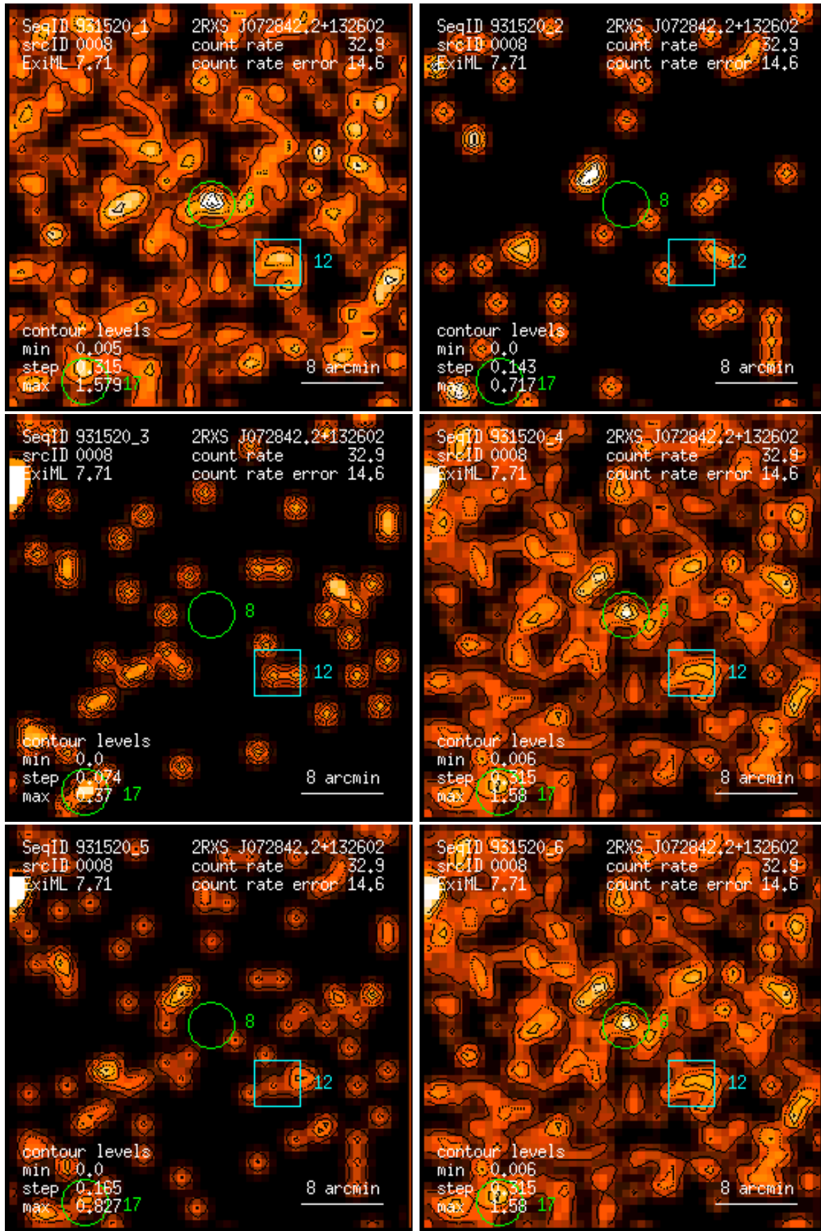
Figure 8: RASS 931520: detection 0008: band rate images, Gaussian filter: (1) PSPC channels 11 – 41, (2) 52 – 90, (3) 91 – 201, (4) 11 – 235, (5) 52 – 201, (6) 11 – 201. Broad band rates in counts/ks. Band rate contour levels in counts/ks/arcmin 2 .
