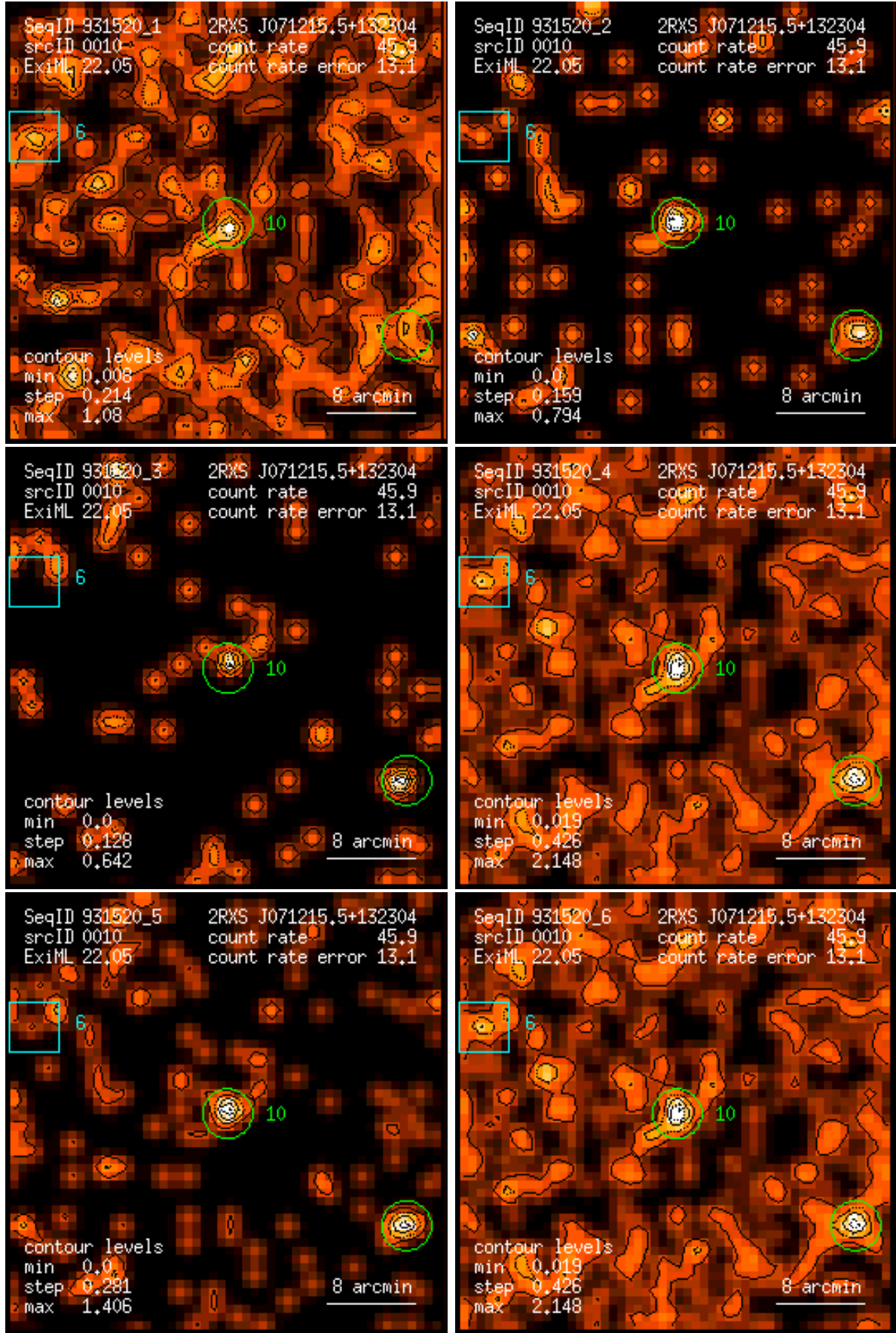
Figure 10: RASS 931520: detection 0010: band rate images, Gaussian filter: (1) PSPC channels 11 – 41, (2) 52 – 90, (3) 91 – 201, (4) 11 – 235, (5) 52 – 201, (6) 11 – 201. Broad band rates in counts/ks. Band rate contour levels in counts/ks/arcmin 2 .
