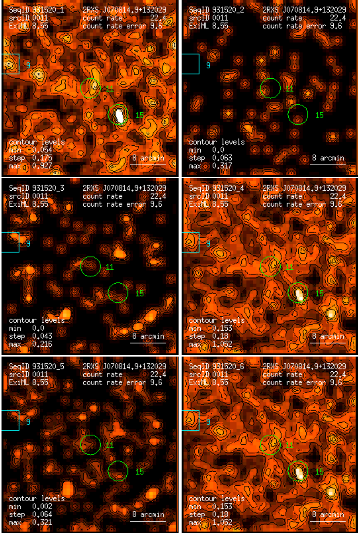
Figure 11: RASS 931520: detection 0011: band rate images, Gaussian filter: (1) PSPC channels 11 – 41, (2) 52 – 90, (3) 91 – 201, (4) 11 – 235, (5) 52 – 201, (6) 11 – 201. Broad band rates in counts/ks. Band rate contour levels in counts/ks/arcmin 2 .
