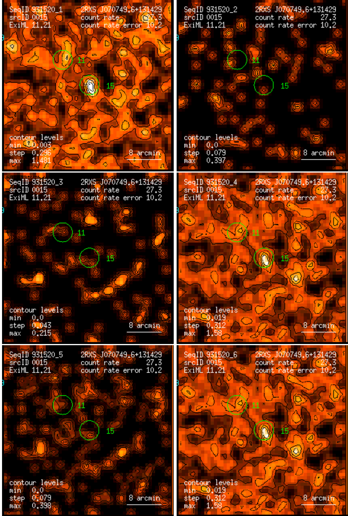
Figure 15: RASS 931520: detection 0015: band rate images, Gaussian filter: (1) PSPC channels 11 – 41, (2) 52 – 90, (3) 91 – 201, (4) 11 – 235, (5) 52 – 201, (6) 11 – 201. Broad band rates in counts/ks. Band rate contour levels in counts/ks/arcmin 2 .
