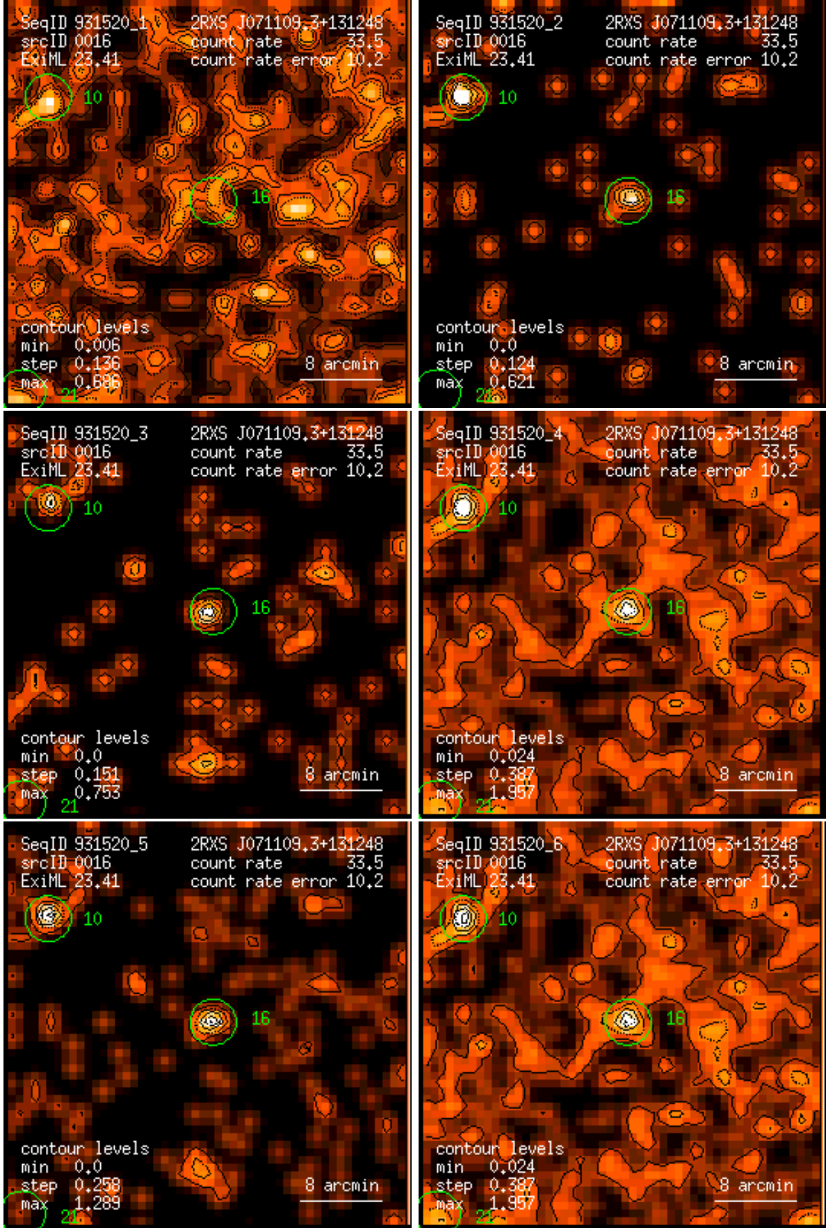
Figure 16: RASS 931520: detection 0016: band rate images, Gaussian filter: (1) PSPC channels 11 – 41, (2) 52 – 90, (3) 91 – 201, (4) 11 – 235, (5) 52 – 201, (6) 11 – 201. Broad band rates in counts/ks. Band rate contour levels in counts/ks/arcmin 2 .
