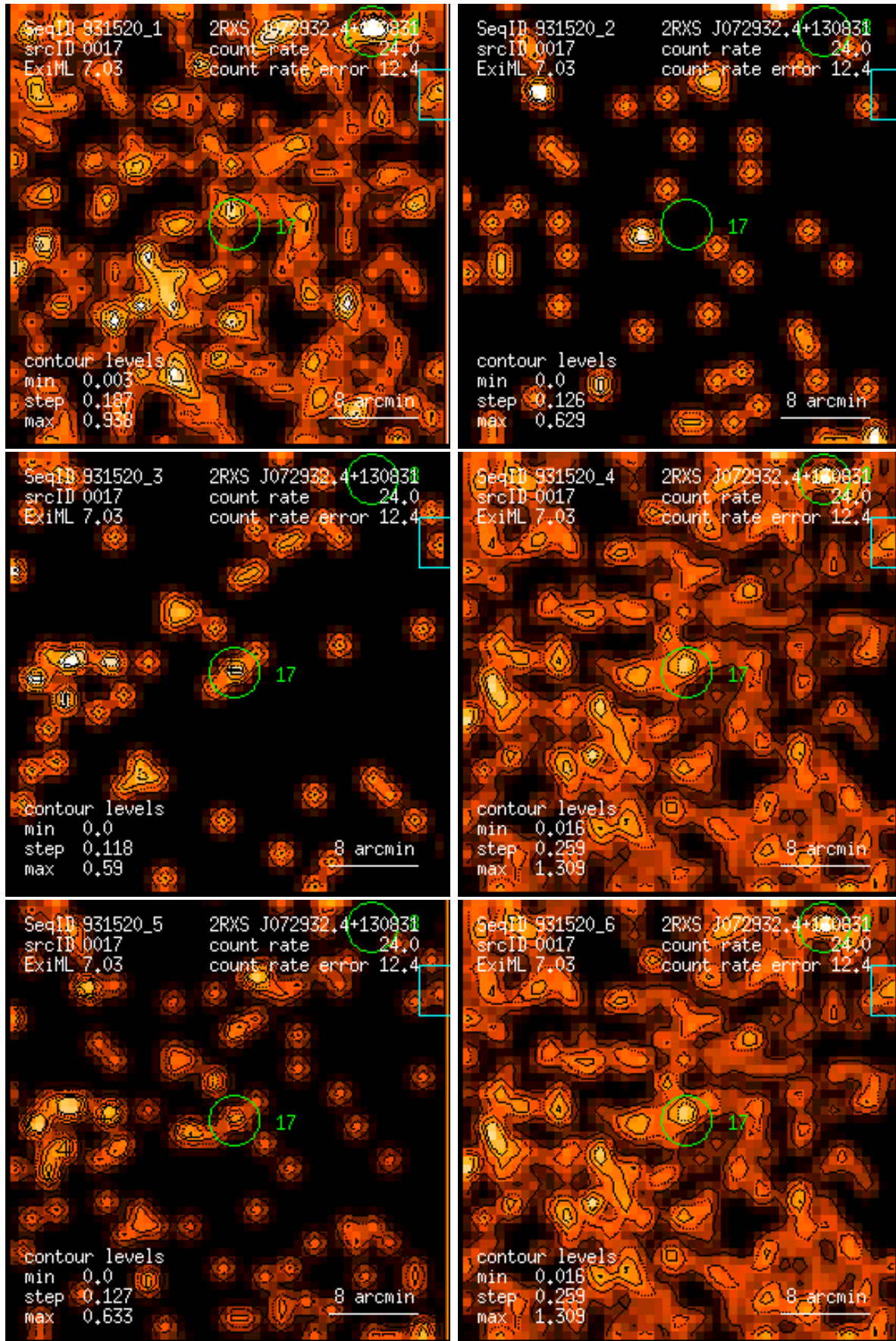
Figure 17: RASS 931520: detection 0017: band rate images, Gaussian filter: (1) PSPC channels 11 – 41, (2) 52 – 90, (3) 91 – 201, (4) 11 – 235, (5) 52 – 201, (6) 11 – 201. Broad band rates in counts/ks. Band rate contour levels in counts/ks/arcmin 2 .
