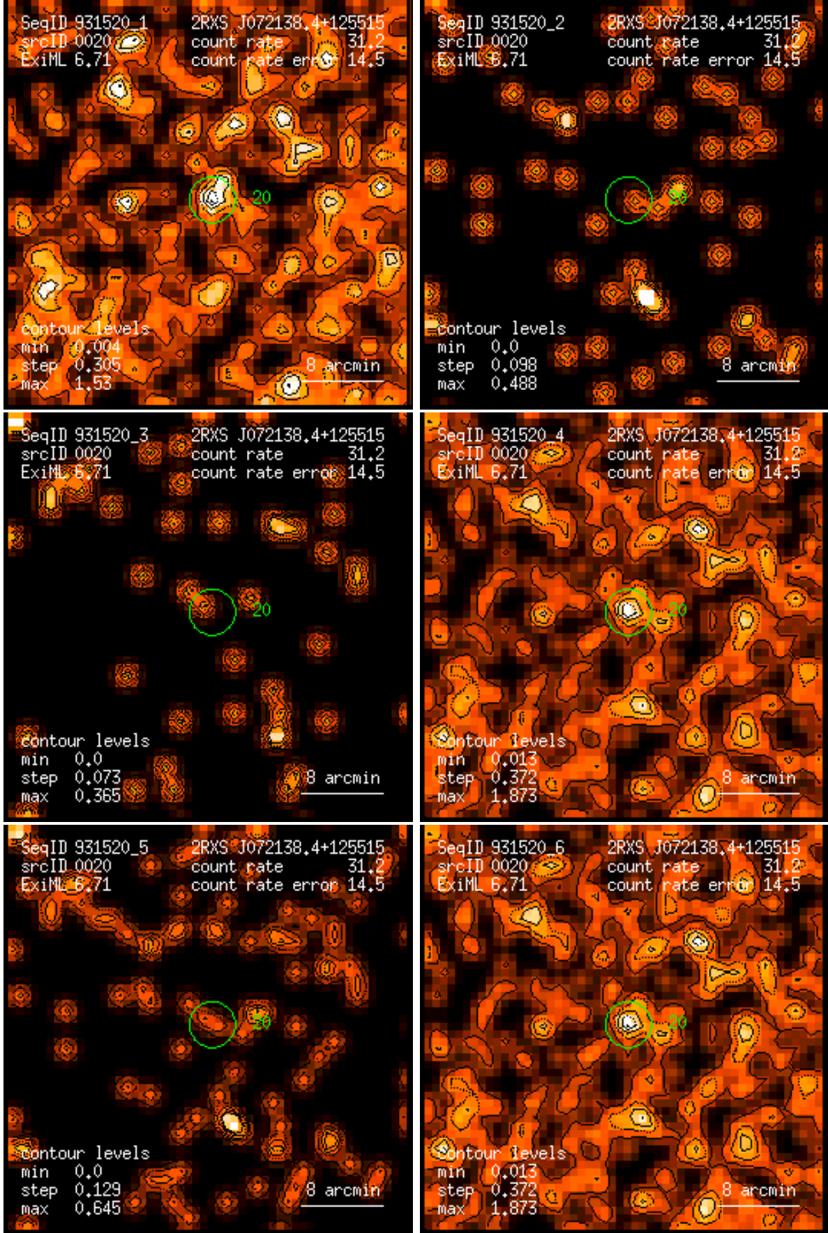
Figure 20: RASS 931520: detection 0020: band rate images, Gaussian filter: (1) PSPC channels 11 – 41, (2) 52 – 90, (3) 91 – 201, (4) 11 – 235, (5) 52 – 201, (6) 11 – 201. Broad band rates in counts/ks. Band rate contour levels in counts/ks/arcmin 2 .
