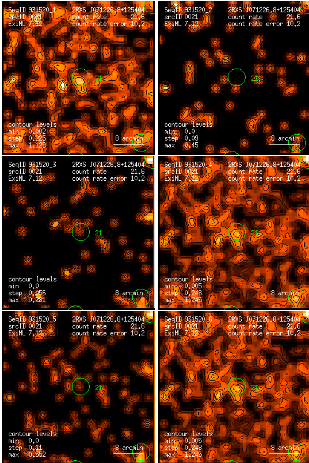
Figure 21: RASS 931520: detection 0021: band rate images, Gaussian filter: (1) PSPC channels 11 – 41, (2) 52 – 90, (3) 91 – 201, (4) 11 – 235, (5) 52 – 201, (6) 11 – 201. Broad band rates in counts/ks. Band rate contour levels in counts/ks/arcmin 2 .
