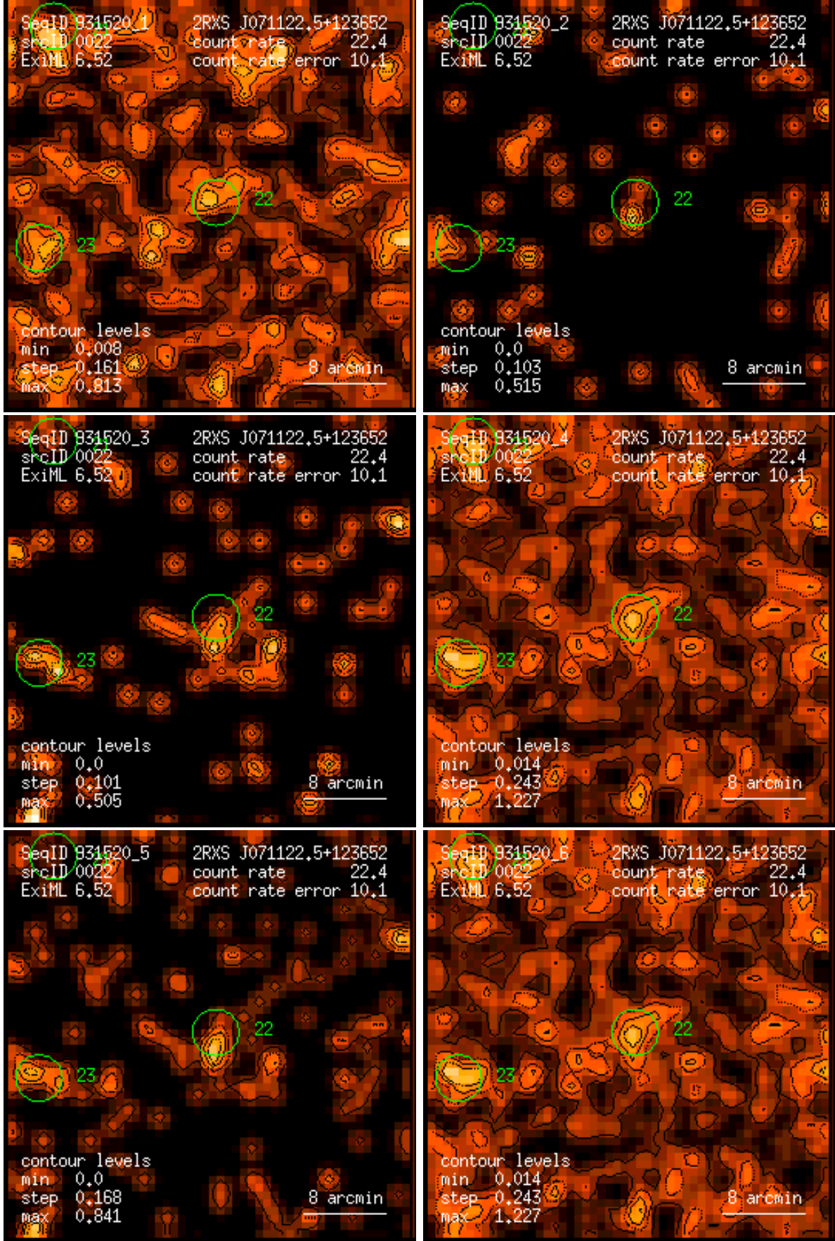
Figure 22: RASS 931520: detection 0022: band rate images, Gaussian filter: (1) PSPC channels 11 – 41, (2) 52 – 90, (3) 91 – 201, (4) 11 – 235, (5) 52 – 201, (6) 11 – 201. Broad band rates in counts/ks. Band rate contour levels in counts/ks/arcmin 2 .
