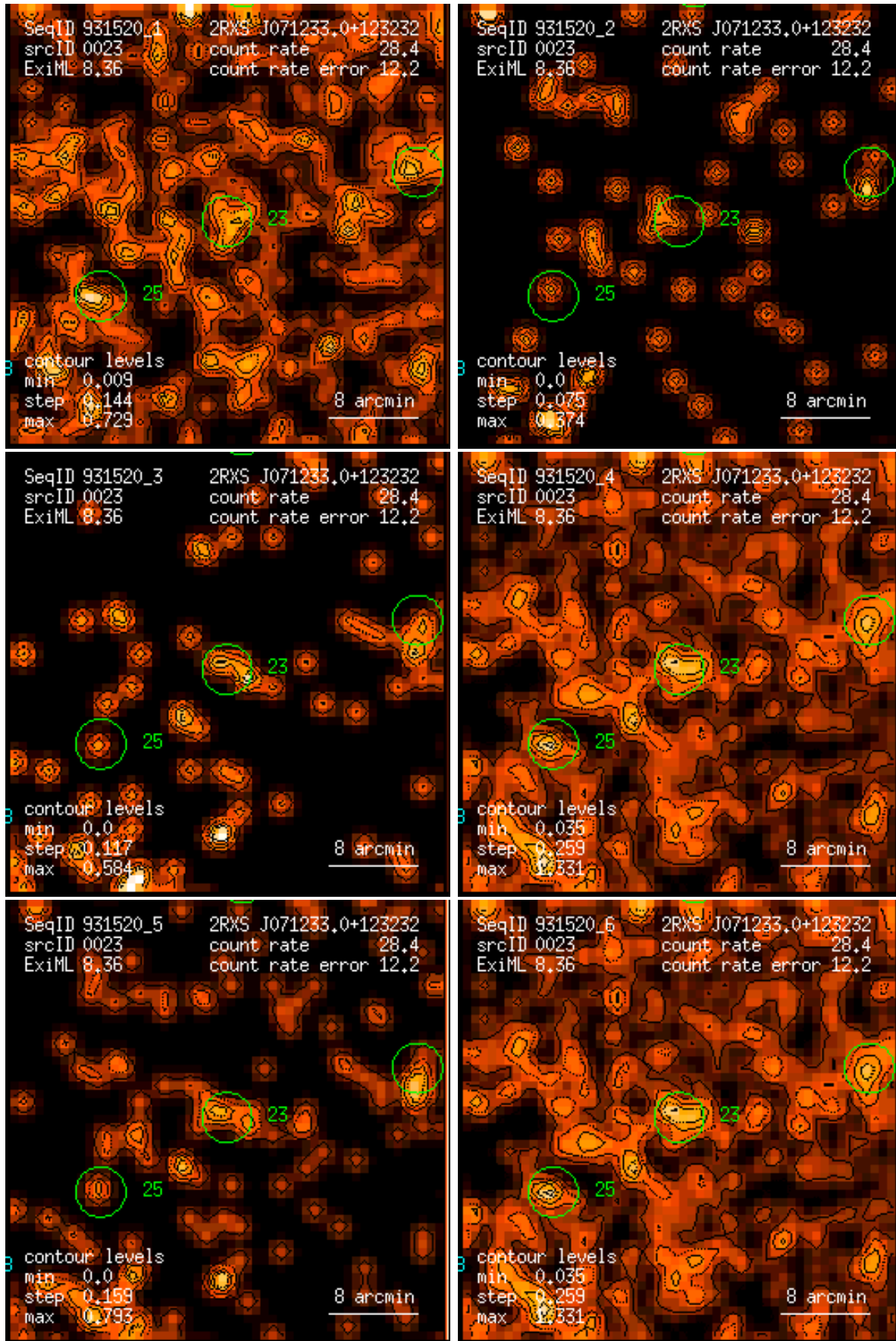
Figure 23: RASS 931520: detection 0023: band rate images, Gaussian filter: (1) PSPC channels 11 – 41, (2) 52 – 90, (3) 91 – 201, (4) 11 – 235, (5) 52 – 201, (6) 11 – 201. Broad band rates in counts/ks. Band rate contour levels in counts/ks/arcmin 2 .
