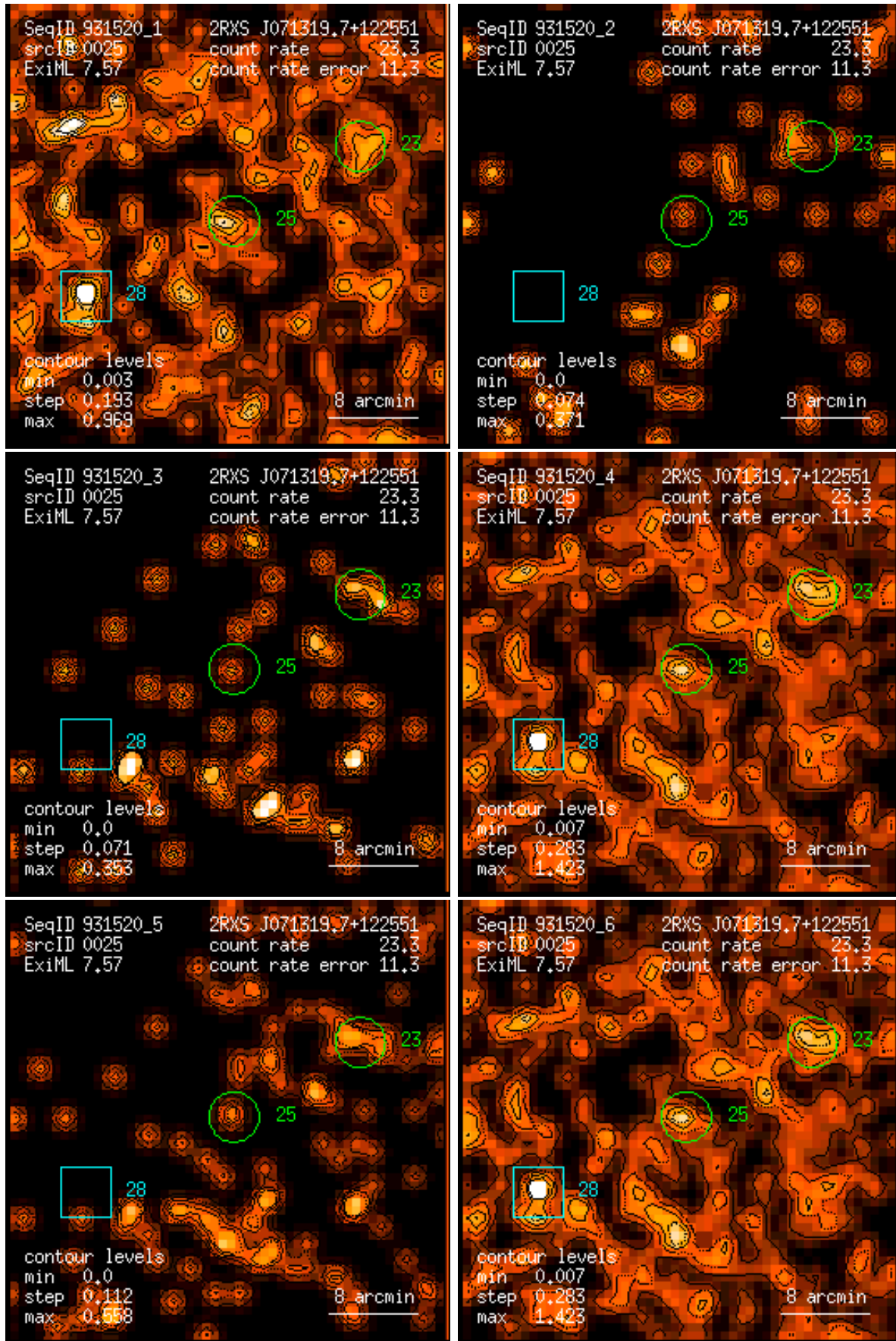
Figure 25: RASS 931520: detection 0025: band rate images, Gaussian filter: (1) PSPC channels 11 – 41, (2) 52 – 90, (3) 91 – 201, (4) 11 – 235, (5) 52 – 201, (6) 11 – 201. Broad band rates in counts/ks. Band rate contour levels in counts/ks/arcmin 2 .
