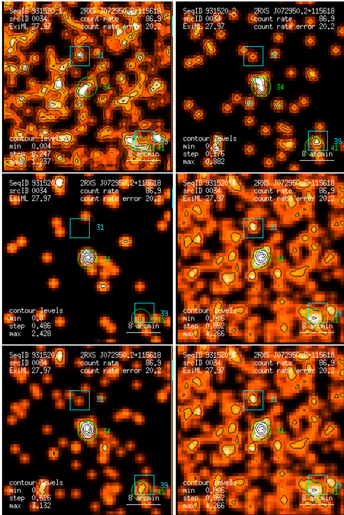
Figure 34: RASS 931520: detection 0034: band rate images, Gaussian filter: (1) PSPC channels 11 – 41, (2) 52 – 90, (3) 91 – 201, (4) 11 – 235, (5) 52 – 201, (6) 11 – 201. Broad band rates in counts/ks. Band rate contour levels in counts/ks/arcmin 2 .
