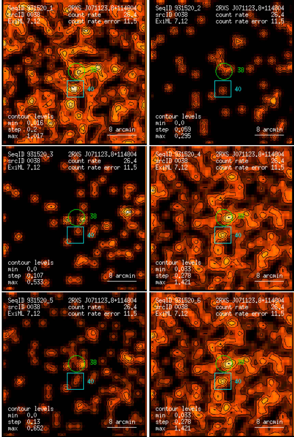
Figure 38: RASS 931520: detection 0038: band rate images, Gaussian filter: (1) PSPC channels 11 – 41, (2) 52 – 90, (3) 91 – 201, (4) 11 – 235, (5) 52 – 201, (6) 11 – 201. Broad band rates in counts/ks. Band rate contour levels in counts/ks/arcmin 2 .
