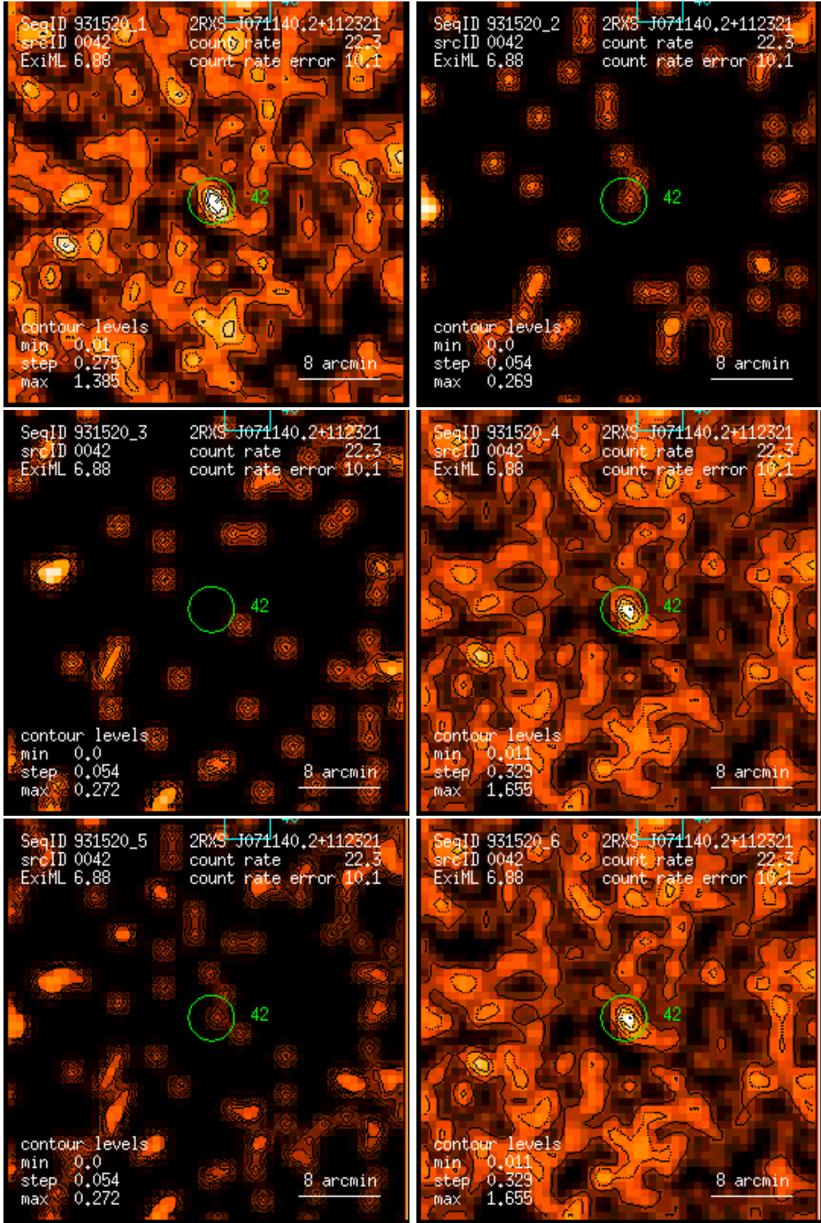
Figure 42: RASS 931520: detection 0042: band rate images, Gaussian filter: (1) PSPC channels 11 – 41, (2) 52 – 90, (3) 91 – 201, (4) 11 – 235, (5) 52 – 201, (6) 11 – 201. Broad band rates in counts/ks. Band rate contour levels in counts/ks/arcmin 2 .
