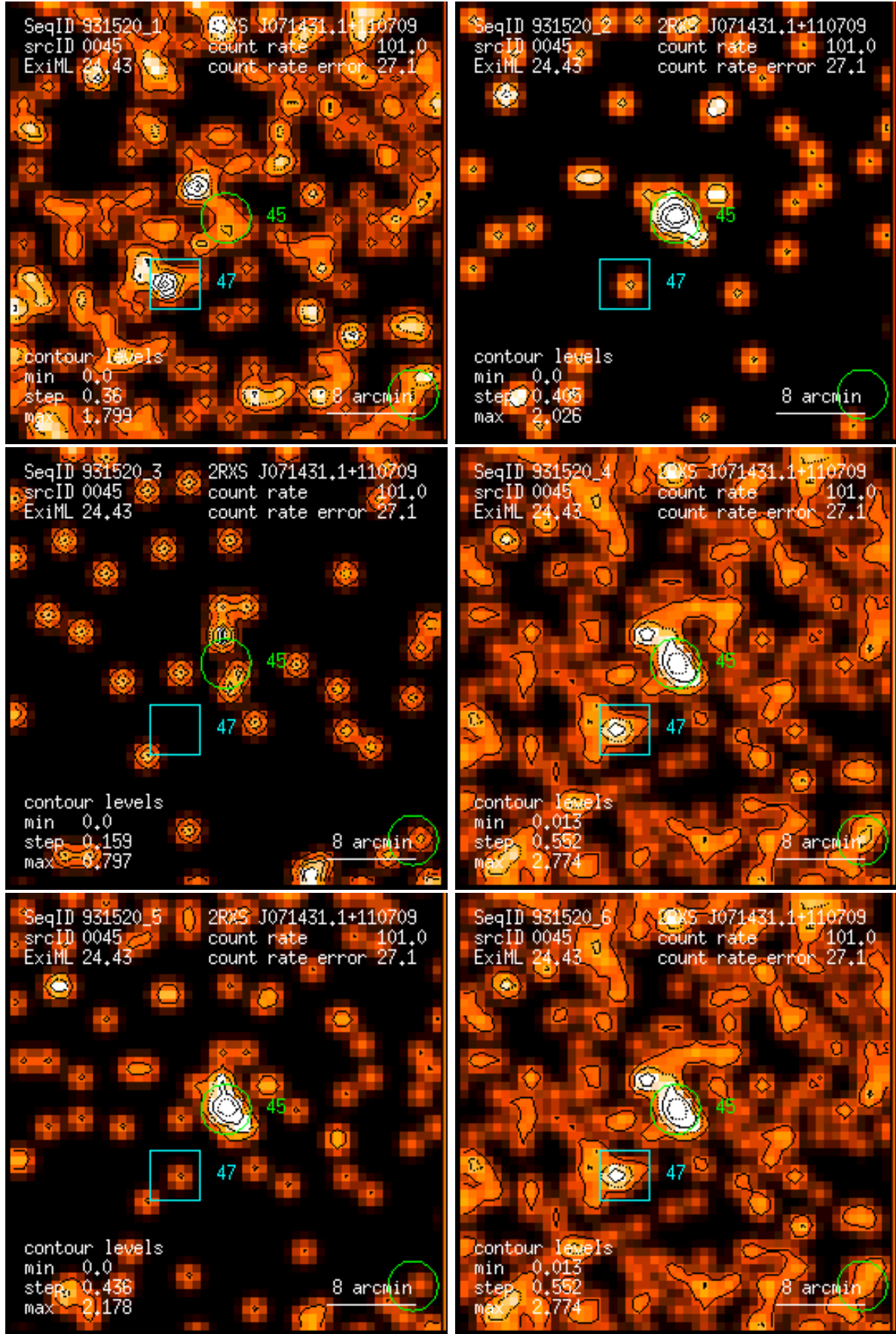
Figure 45: RASS 931520: detection 0045: band rate images, Gaussian filter: (1) PSPC channels 11 – 41, (2) 52 – 90, (3) 91 – 201, (4) 11 – 235, (5) 52 – 201, (6) 11 – 201. Broad band rates in counts/ks. Band rate contour levels in counts/ks/arcmin 2 .
