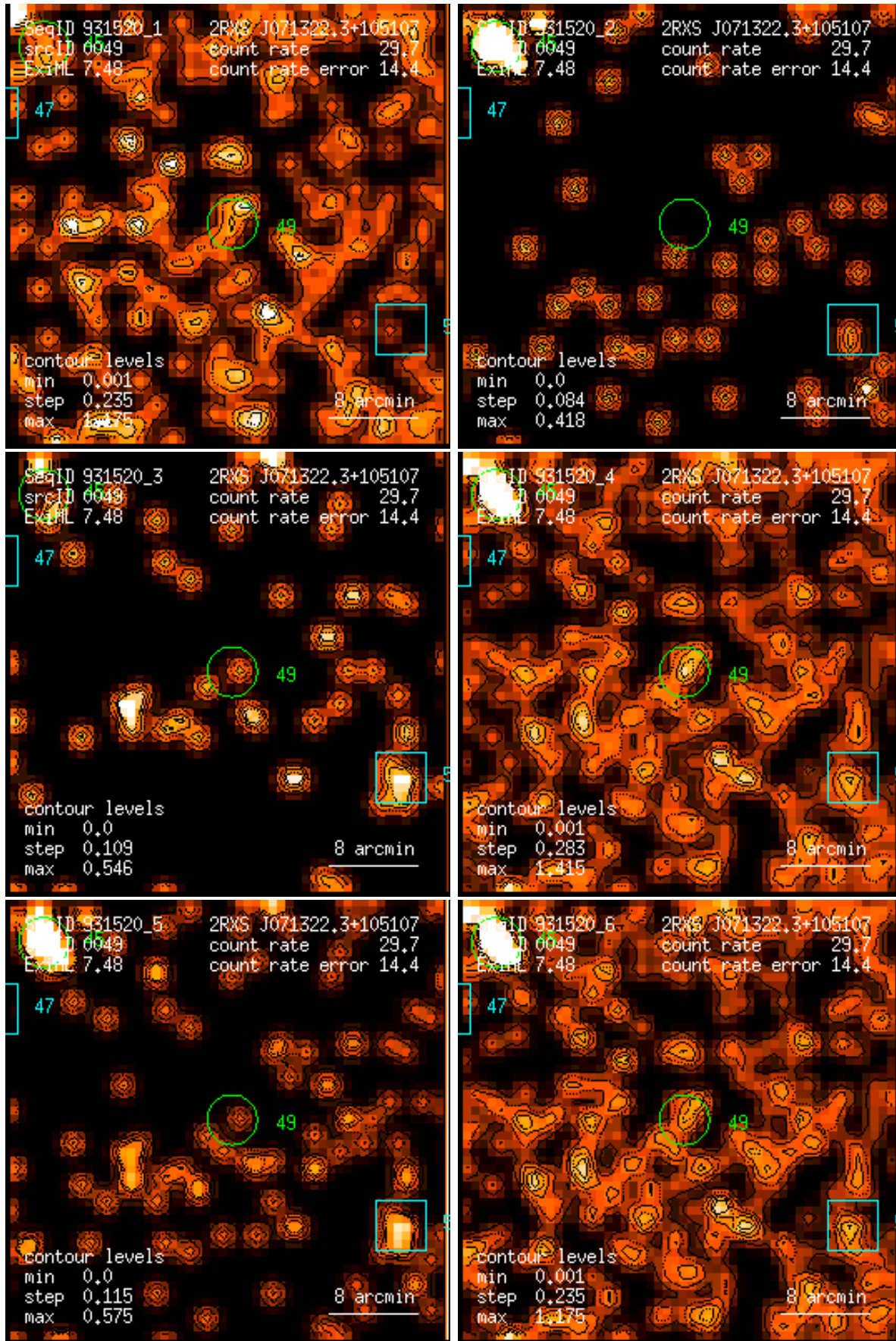
Figure 49: RASS 931520: detection 0049: band rate images, Gaussian filter: (1) PSPC channels 11 – 41, (2) 52 – 90, (3) 91 – 201, (4) 11 – 235, (5) 52 – 201, (6) 11 – 201. Broad band rates in counts/ks. Band rate contour levels in counts/ks/arcmin 2 .
